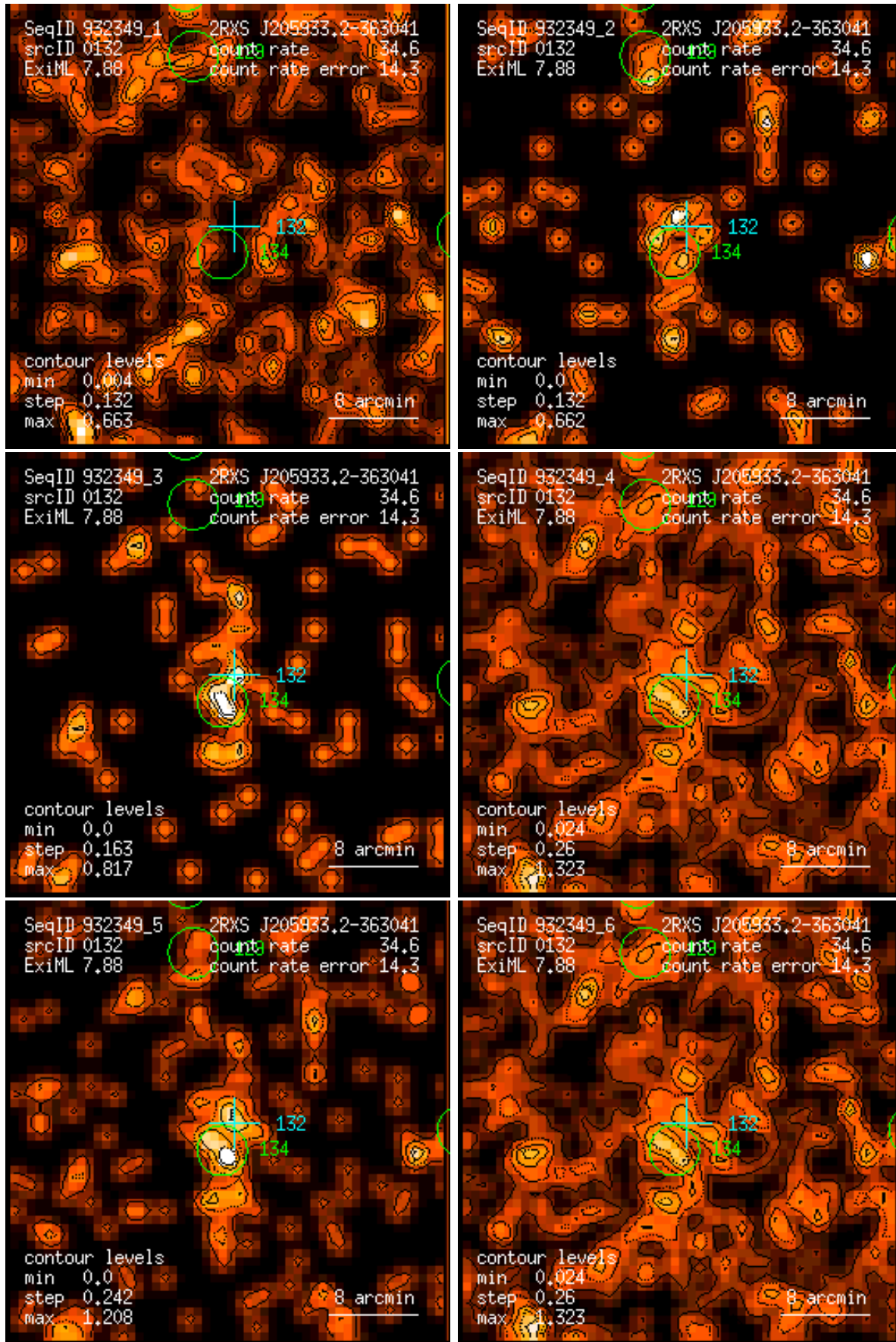
Figure 132: RASS 932349: detection 0132: band rate images, Gaussian filter: (1) PSPC channels 11 – 41, (2) 52 – 90, (3) 91 – 201, (4) 11 – 235, (5) 52 – 201, (6) 11 – 201. Broad band rates in counts/ks. Band rate contour levels in counts/ks/arcmin 2 .
