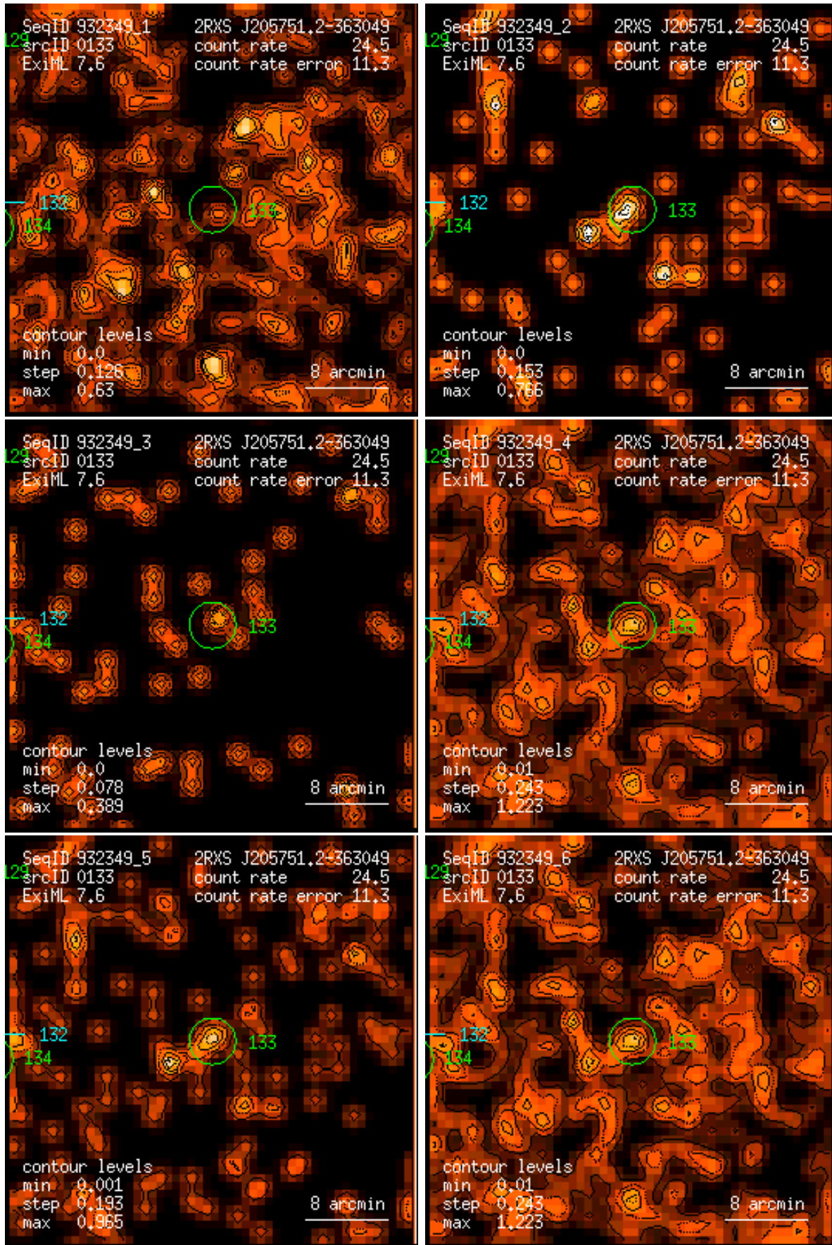
Figure 133: RASS 932349: detection 0133: band rate images, Gaussian filter: (1) PSPC channels 11 – 41, (2) 52 – 90, (3) 91 – 201, (4) 11 – 235, (5) 52 – 201, (6) 11 – 201. Broad band rates in counts/ks. Band rate contour levels in counts/ks/arcmin 2 .
