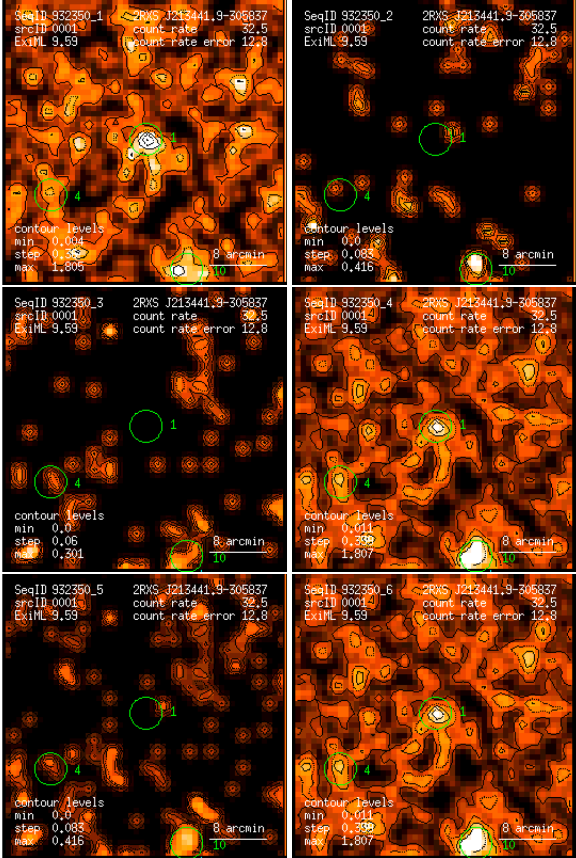
Figure 1: RASS 932350: detection 0001: band rate images, Gaussian filter: (1) PSPC channels 11 – 41, (2) 52 – 90, (3) 91 – 201, (4) 11 – 235, (5) 52 – 201, (6) 11 – 201. Broad band rates in counts/ks. Band rate contour levels in counts/ks/arcmin 2 .
