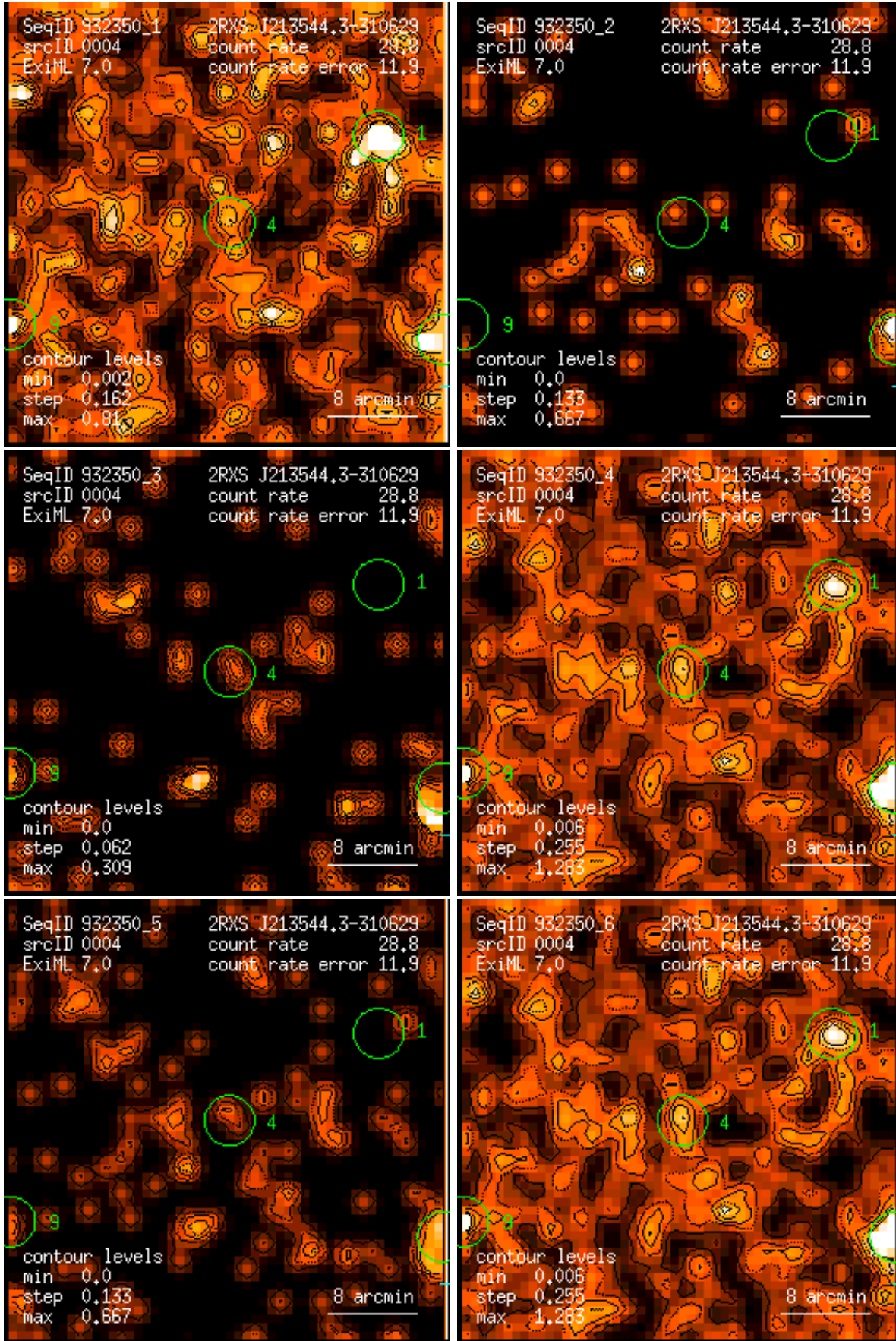
Figure 4: RASS 932350: detection 0004: band rate images, Gaussian filter: (1) PSPC channels 11 – 41, (2) 52 – 90, (3) 91 – 201, (4) 11 – 235, (5) 52 – 201, (6) 11 – 201. Broad band rates in counts/ks. Band rate contour levels in counts/ks/arcmin 2 .
