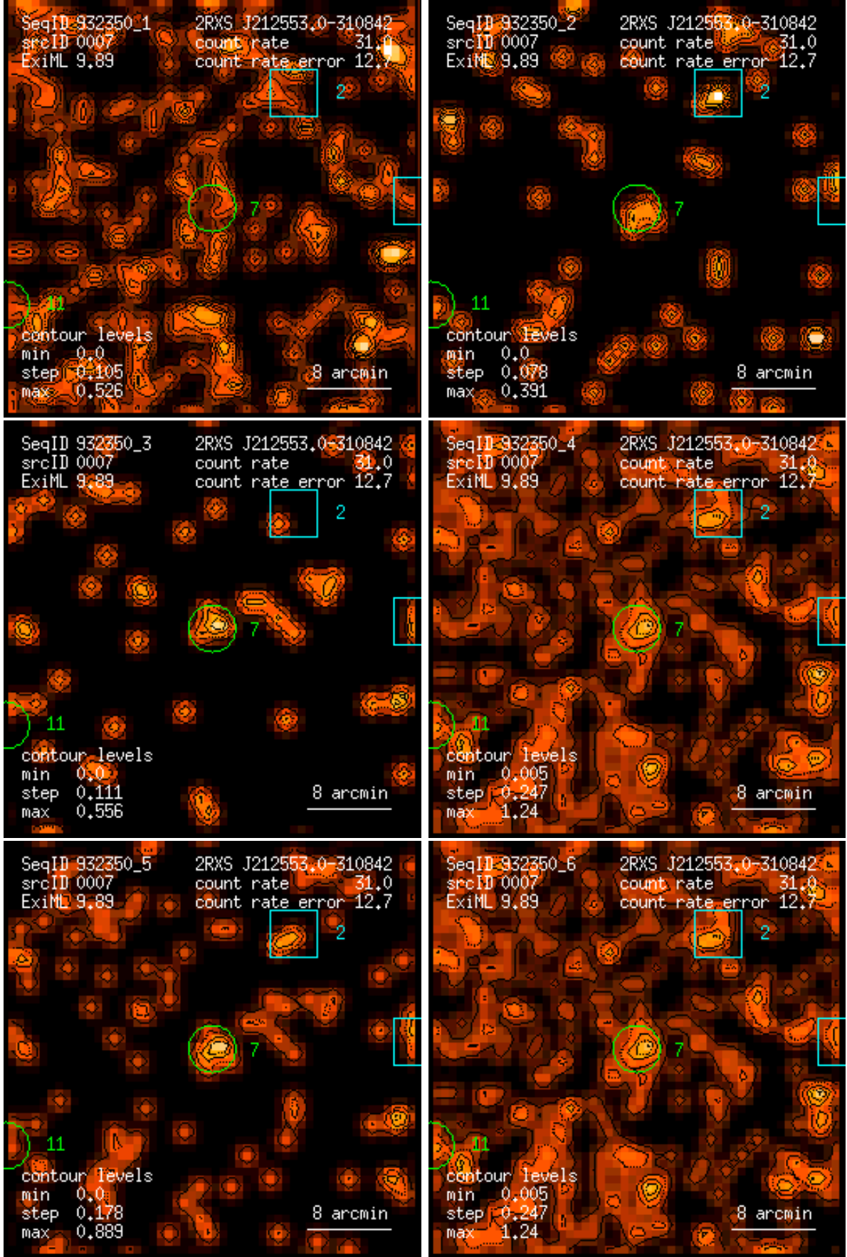
Figure 7: RASS 932350: detection 0007: band rate images, Gaussian filter: (1) PSPC channels 11 – 41, (2) 52 – 90, (3) 91 – 201, (4) 11 – 235, (5) 52 – 201, (6) 11 – 201. Broad band rates in counts/ks. Band rate contour levels in counts/ks/arcmin 2 .
