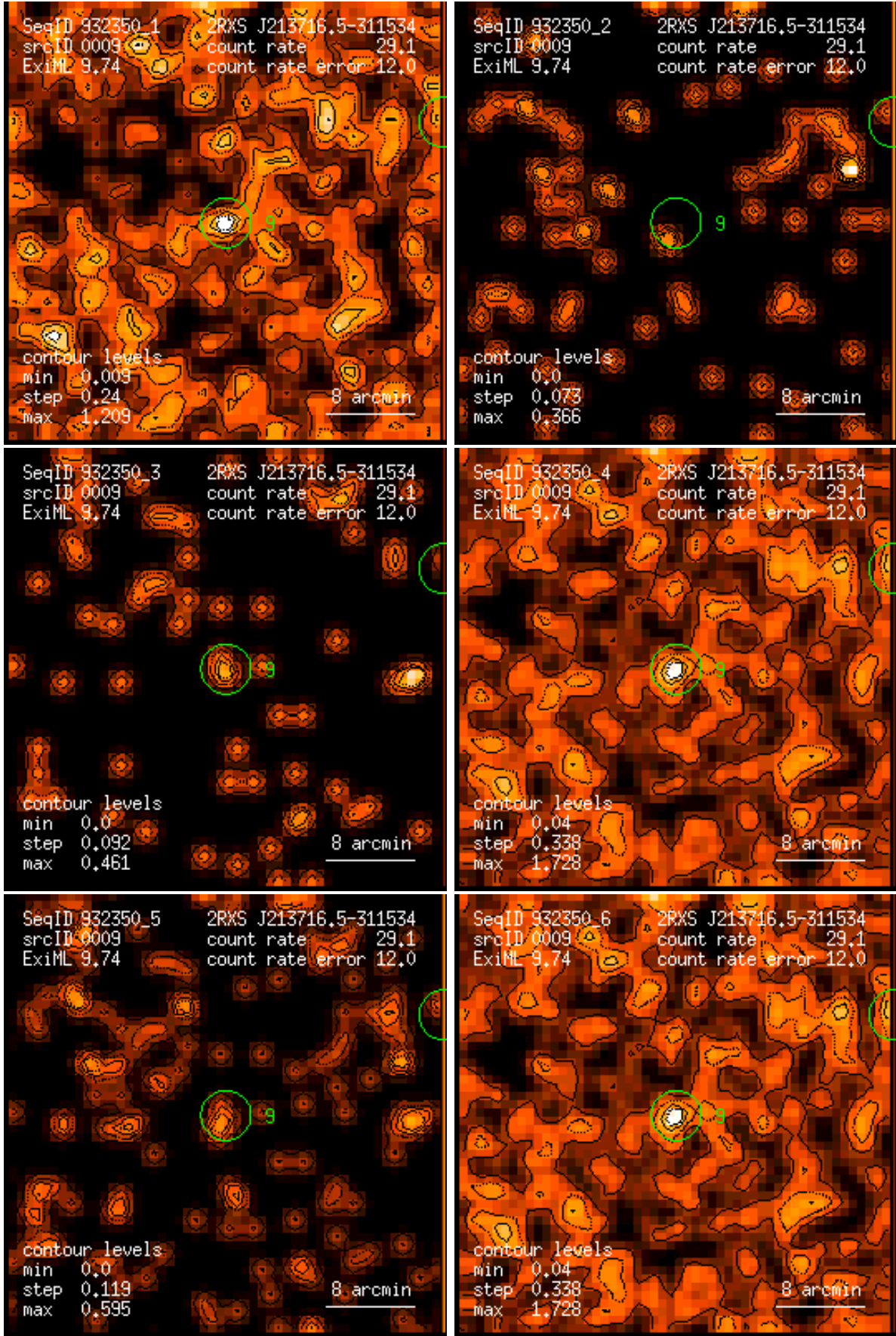
Figure 9: RASS 932350: detection 0009: band rate images, Gaussian filter: (1) PSPC channels 11 – 41, (2) 52 – 90, (3) 91 – 201, (4) 11 – 235, (5) 52 – 201, (6) 11 – 201. Broad band rates in counts/ks. Band rate contour levels in counts/ks/arcmin 2 .
