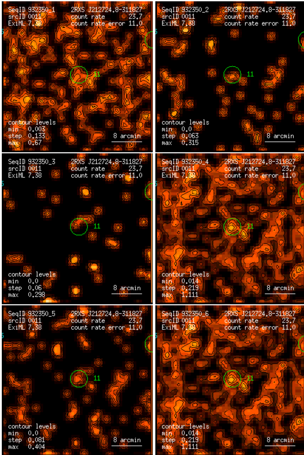
Figure 11: RASS 932350: detection 0011: band rate images, Gaussian filter: (1) PSPC channels 11 – 41, (2) 52 – 90, (3) 91 – 201, (4) 11 – 235, (5) 52 – 201, (6) 11 – 201. Broad band rates in counts/ks. Band rate contour levels in counts/ks/arcmin 2 .
