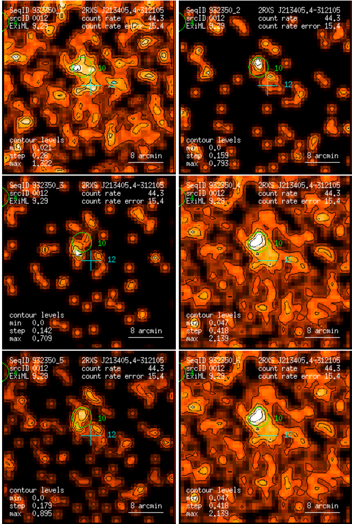
Figure 12: RASS 932350: detection 0012: band rate images, Gaussian filter: (1) PSPC channels 11 – 41, (2) 52 – 90, (3) 91 – 201, (4) 11 – 235, (5) 52 – 201, (6) 11 – 201. Broad band rates in counts/ks. Band rate contour levels in counts/ks/arcmin 2 .
