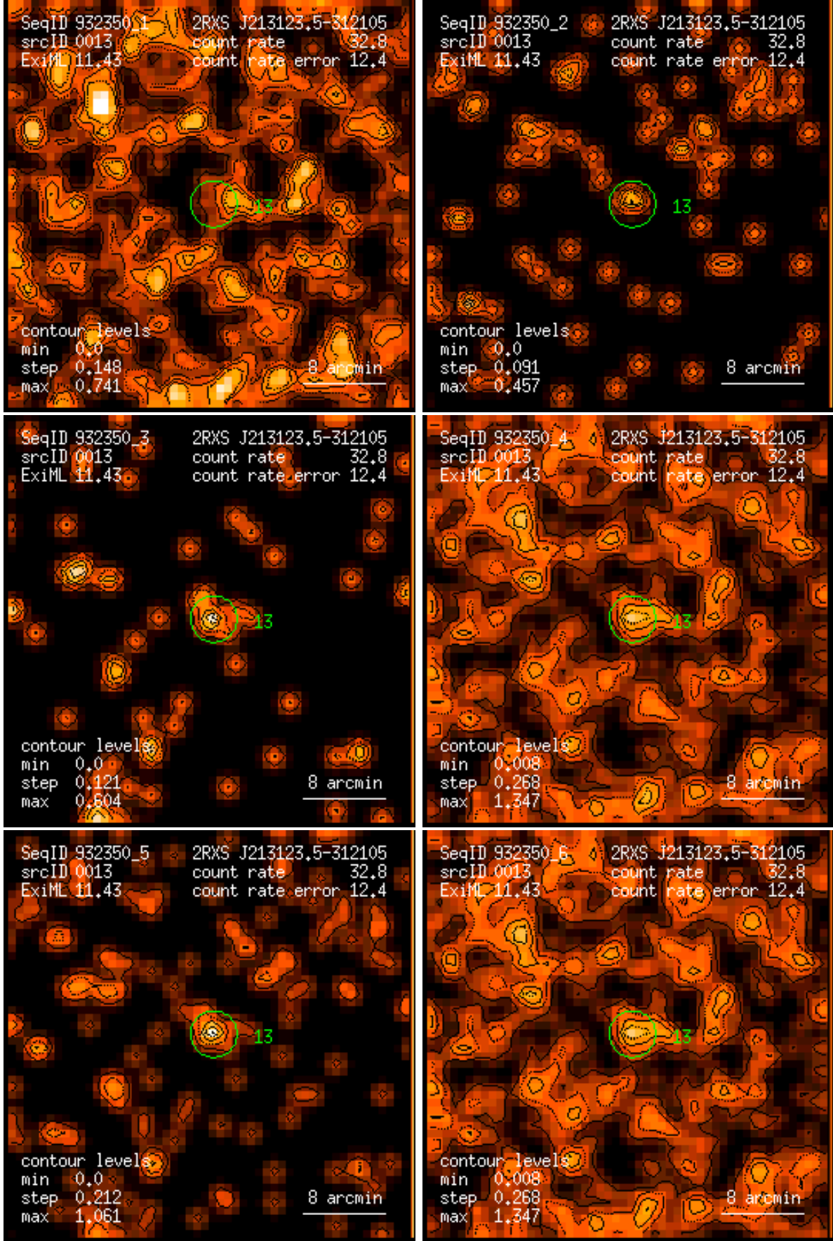
Figure 13: RASS 932350: detection 0013: band rate images, Gaussian filter: (1) PSPC channels 11 – 41, (2) 52 – 90, (3) 91 – 201, (4) 11 – 235, (5) 52 – 201, (6) 11 – 201. Broad band rates in counts/ks. Band rate contour levels in counts/ks/arcmin 2 .
