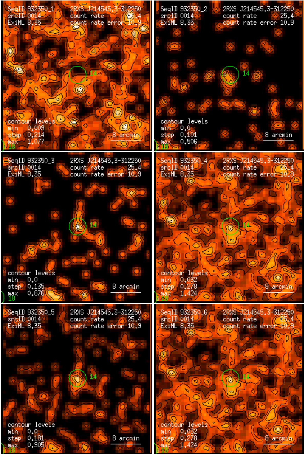
Figure 14: RASS 932350: detection 0014: band rate images, Gaussian filter: (1) PSPC channels 11 – 41, (2) 52 – 90, (3) 91 – 201, (4) 11 – 235, (5) 52 – 201, (6) 11 – 201. Broad band rates in counts/ks. Band rate contour levels in counts/ks/arcmin 2 .
