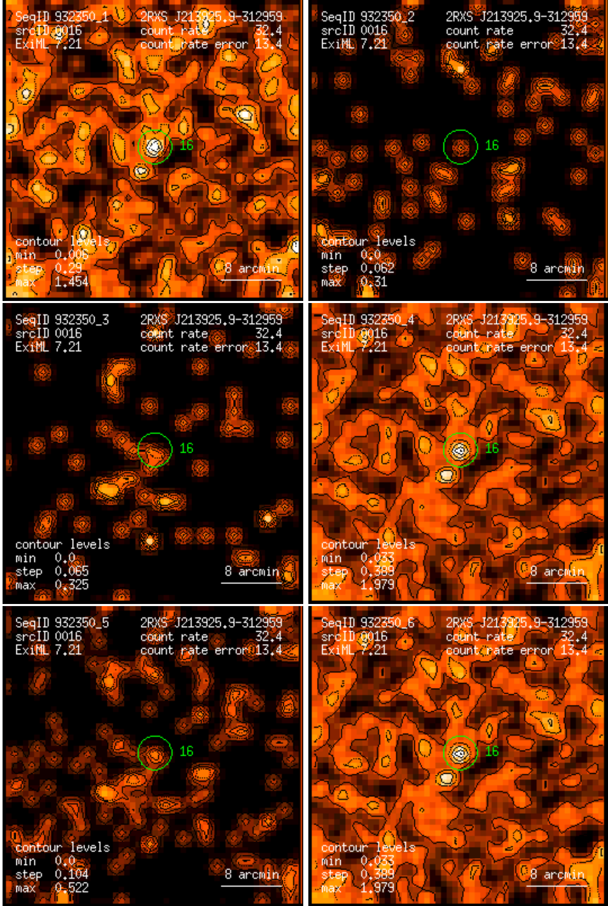
Figure 16: RASS 932350: detection 0016: band rate images, Gaussian filter: (1) PSPC channels 11 – 41, (2) 52 – 90, (3) 91 – 201, (4) 11 – 235, (5) 52 – 201, (6) 11 – 201. Broad band rates in counts/ks. Band rate contour levels in counts/ks/arcmin 2 .
