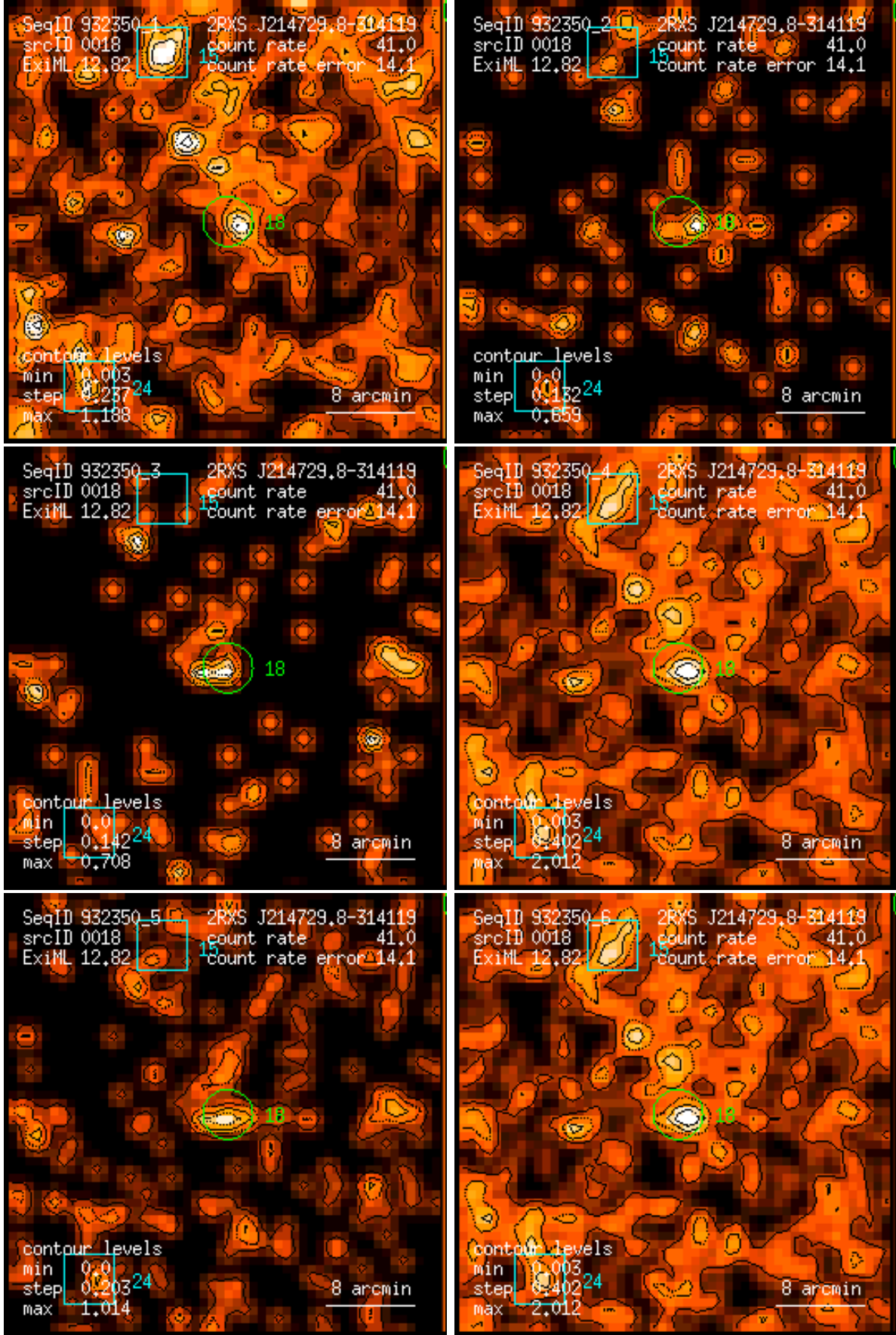
Figure 18: RASS 932350: detection 0018: band rate images, Gaussian filter: (1) PSPC channels 11 – 41, (2) 52 – 90, (3) 91 – 201, (4) 11 – 235, (5) 52 – 201, (6) 11 – 201. Broad band rates in counts/ks. Band rate contour levels in counts/ks/arcmin 2 .
