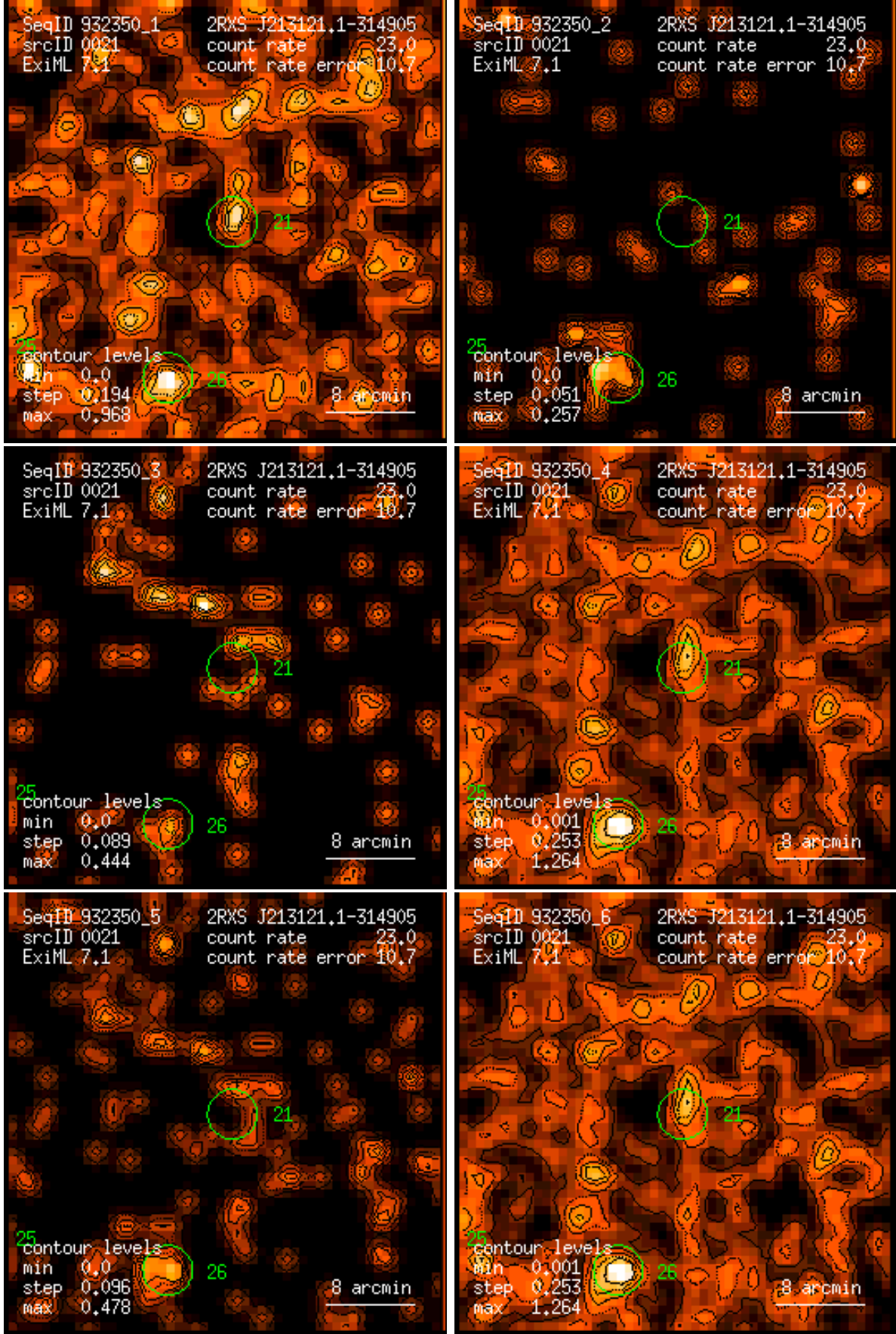
Figure 21: RASS 932350: detection 0021: band rate images, Gaussian filter: (1) PSPC channels 11 – 41, (2) 52 – 90, (3) 91 – 201, (4) 11 – 235, (5) 52 – 201, (6) 11 – 201. Broad band rates in counts/ks. Band rate contour levels in counts/ks/arcmin 2 .
