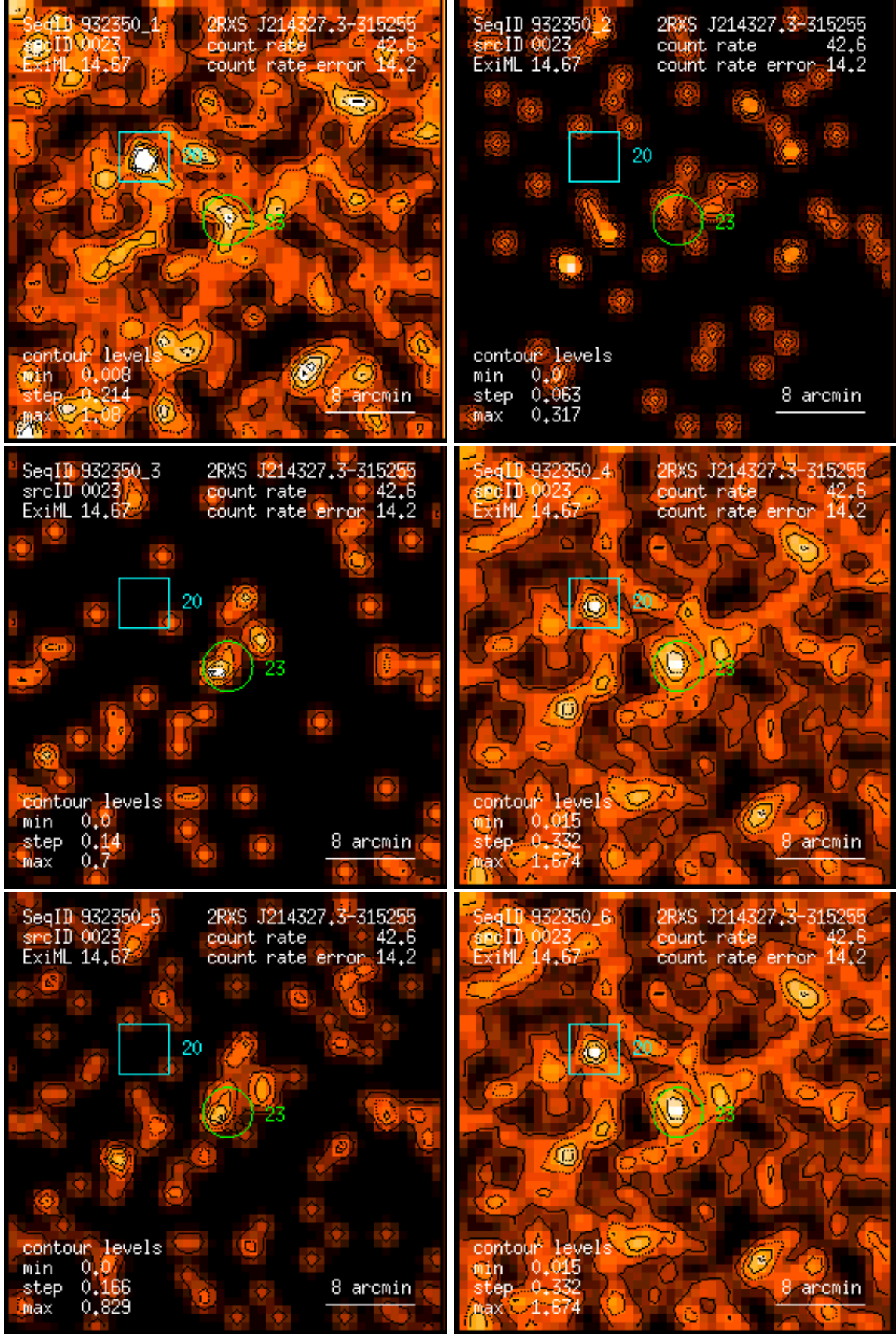
Figure 23: RASS 932350: detection 0023: band rate images, Gaussian filter: (1) PSPC channels 11 – 41, (2) 52 – 90, (3) 91 – 201, (4) 11 – 235, (5) 52 – 201, (6) 11 – 201. Broad band rates in counts/ks. Band rate contour levels in counts/ks/arcmin 2 .
