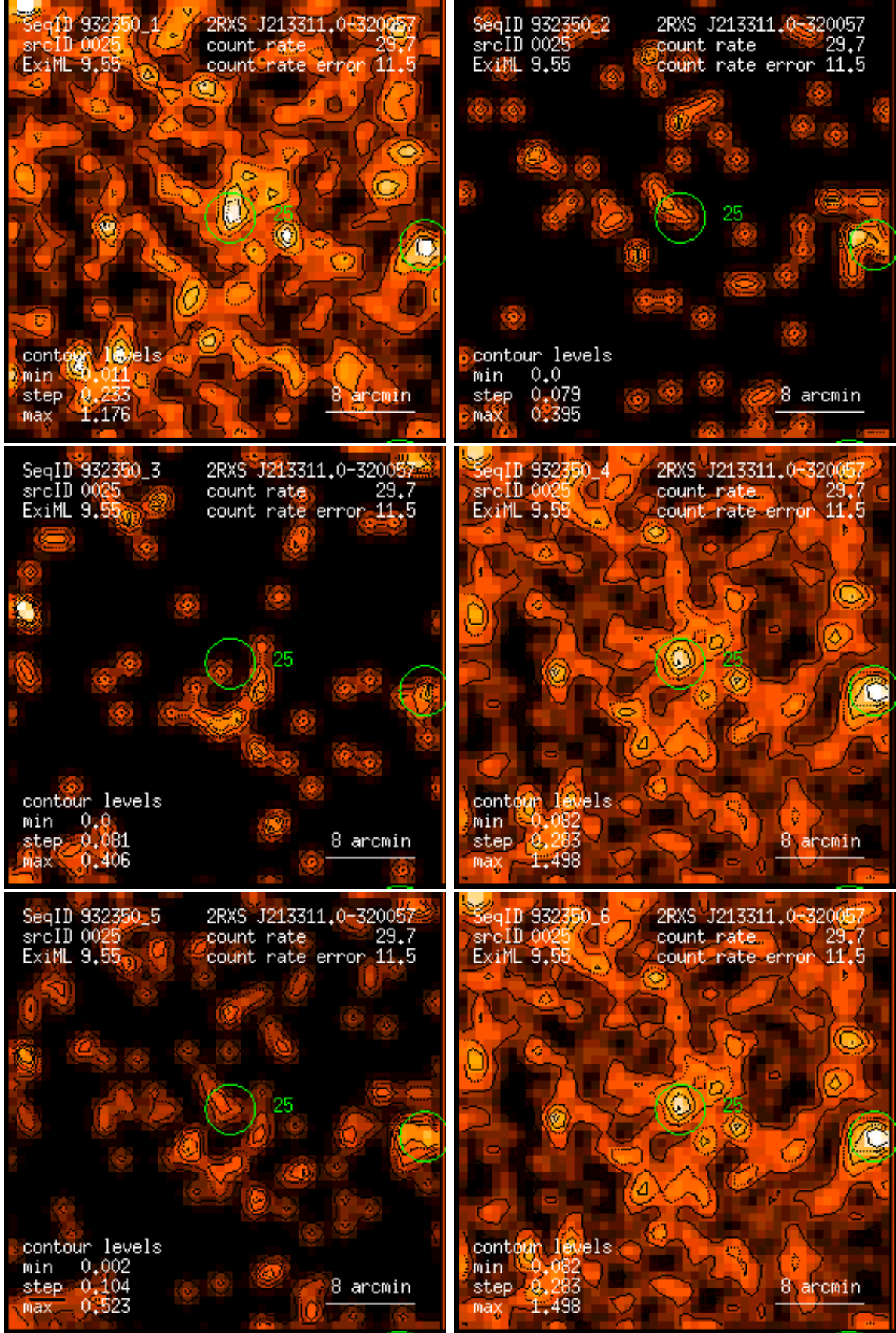
Figure 25: RASS 932350: detection 0025: band rate images, Gaussian filter: (1) PSPC channels 11 – 41, (2) 52 – 90, (3) 91 – 201, (4) 11 – 235, (5) 52 – 201, (6) 11 – 201. Broad band rates in counts/ks. Band rate contour levels in counts/ks/arcmin 2 .
