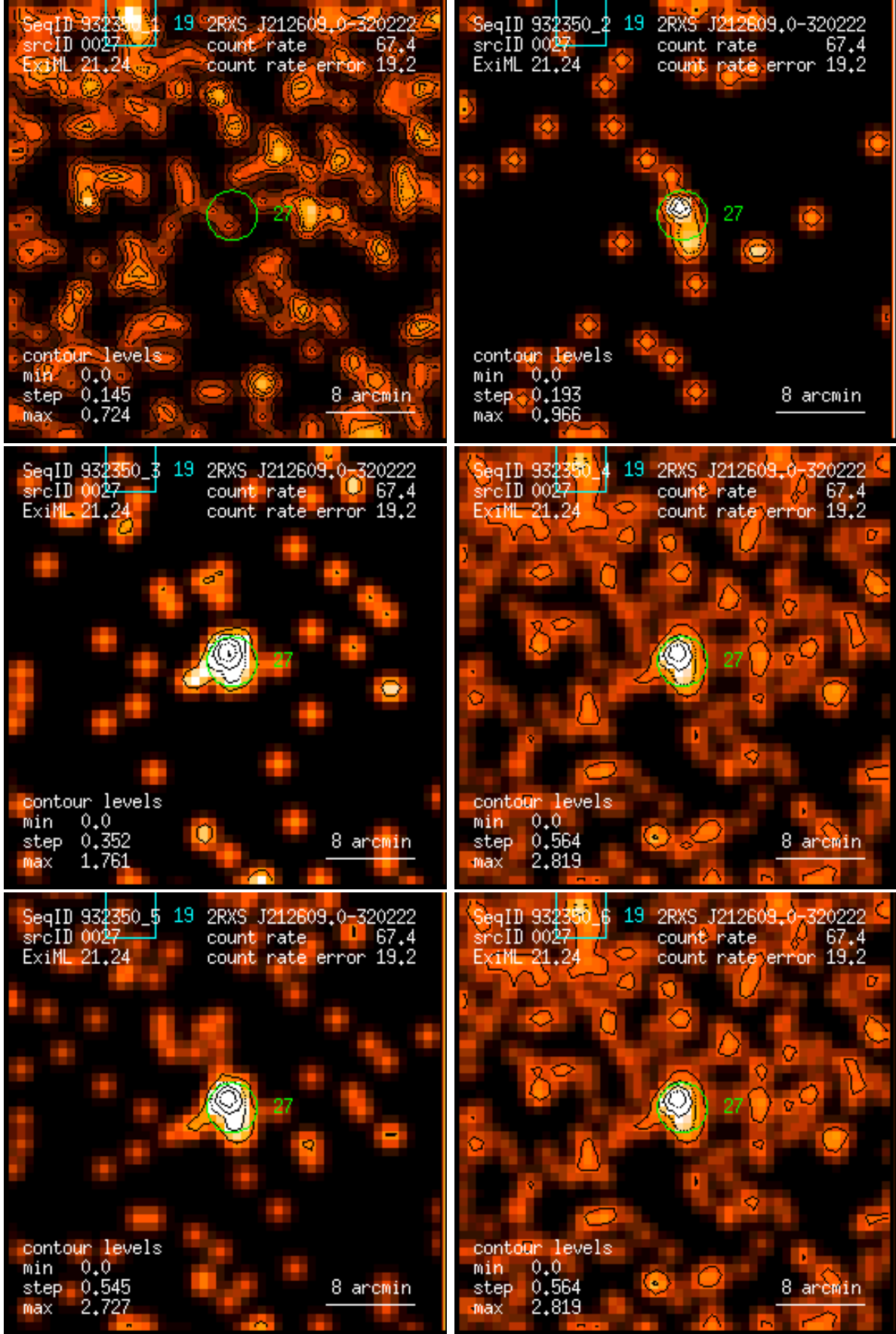
Figure 27: RASS 932350: detection 0027: band rate images, Gaussian filter: (1) PSPC channels 11 – 41, (2) 52 – 90, (3) 91 – 201, (4) 11 – 235, (5) 52 – 201, (6) 11 – 201. Broad band rates in counts/ks. Band rate contour levels in counts/ks/arcmin 2 .
