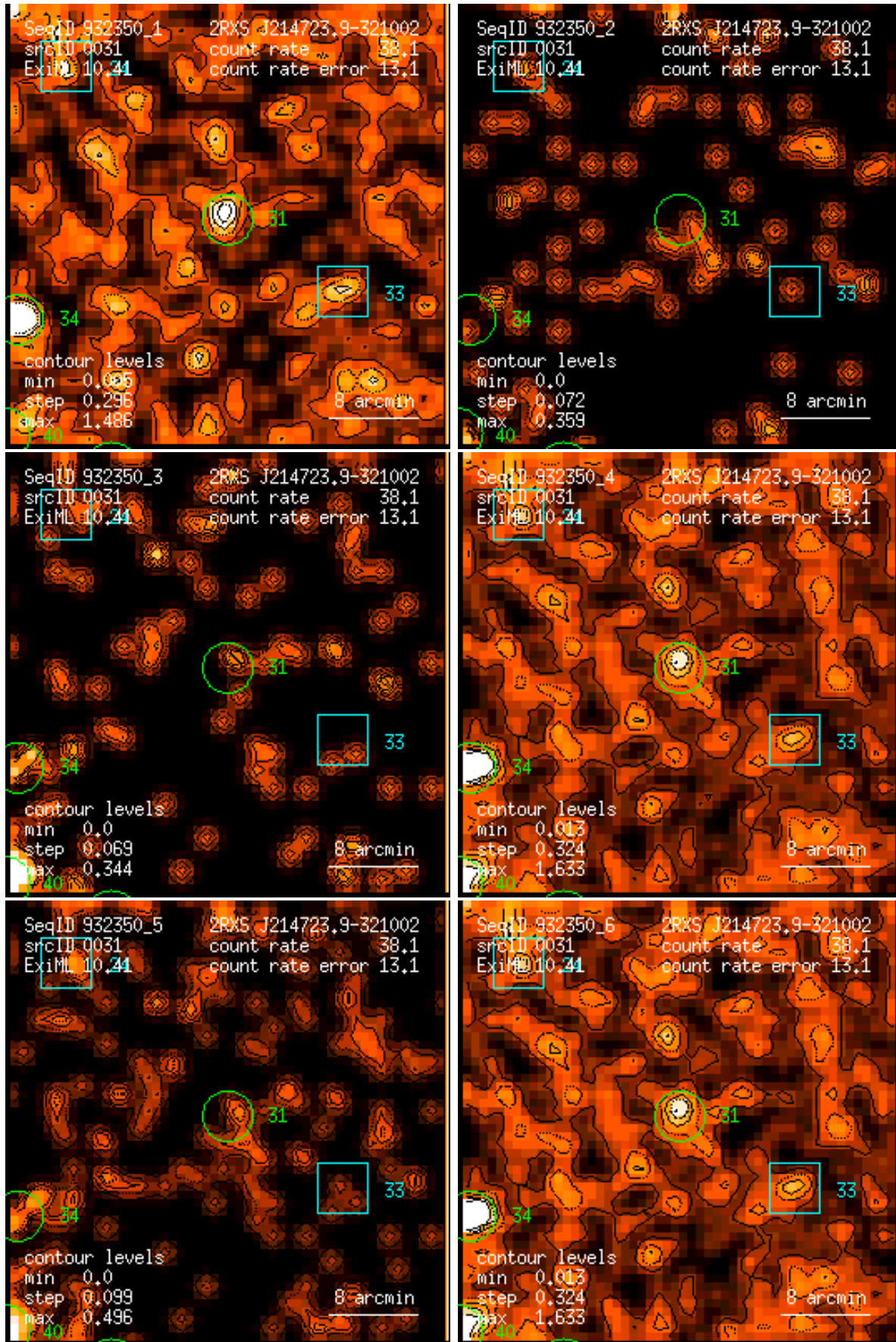
Figure 31: RASS 932350: detection 0031: band rate images, Gaussian filter: (1) PSPC channels 11 – 41, (2) 52 – 90, (3) 91 – 201, (4) 11 – 235, (5) 52 – 201, (6) 11 – 201. Broad band rates in counts/ks. Band rate contour levels in counts/ks/arcmin 2 .
