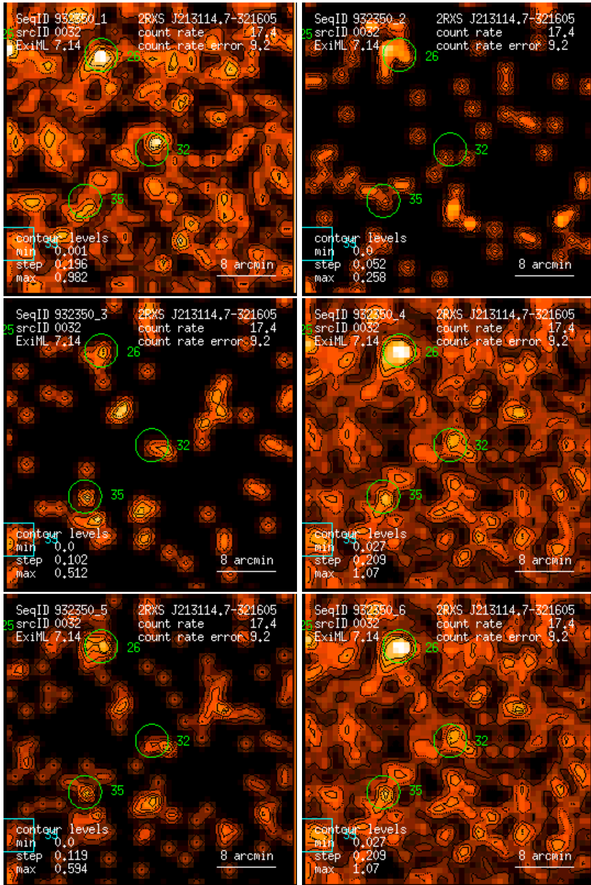
Figure 32: RASS 932350: detection 0032: band rate images, Gaussian filter: (1) PSPC channels 11 – 41, (2) 52 – 90, (3) 91 – 201, (4) 11 – 235, (5) 52 – 201, (6) 11 – 201. Broad band rates in counts/ks. Band rate contour levels in counts/ks/arcmin 2 .
