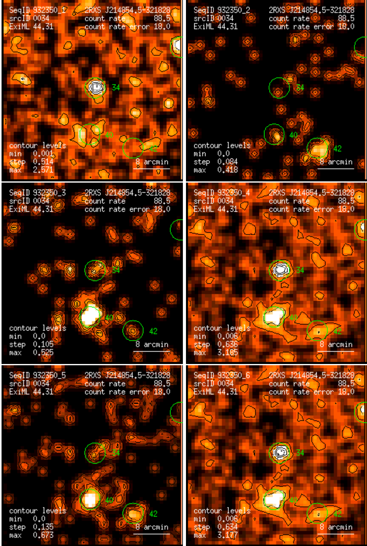
Figure 34: RASS 932350: detection 0034: band rate images, Gaussian filter: (1) PSPC channels 11 – 41, (2) 52 – 90, (3) 91 – 201, (4) 11 – 235, (5) 52 – 201, (6) 11 – 201. Broad band rates in counts/ks. Band rate contour levels in counts/ks/arcmin 2 .
