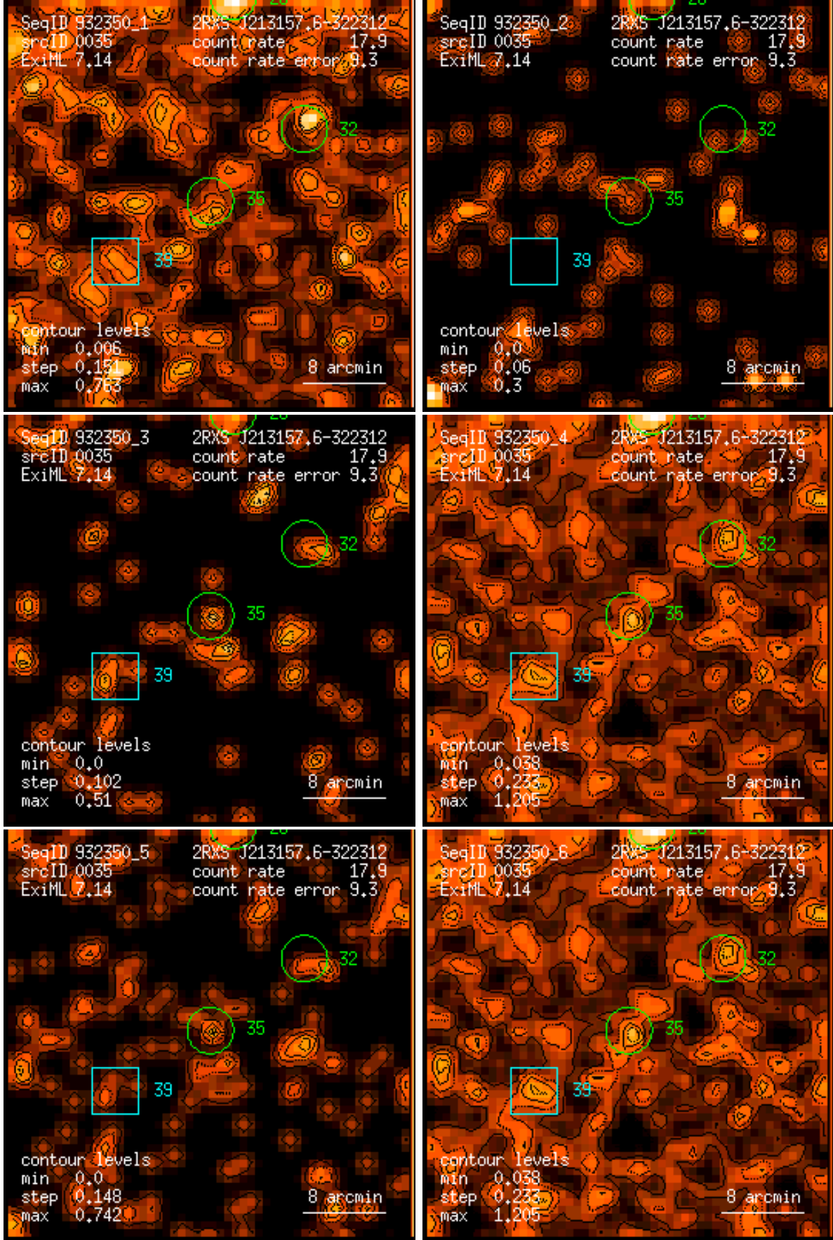
Figure 35: RASS 932350: detection 0035: band rate images, Gaussian filter: (1) PSPC channels 11 – 41, (2) 52 – 90, (3) 91 – 201, (4) 11 – 235, (5) 52 – 201, (6) 11 – 201. Broad band rates in counts/ks. Band rate contour levels in counts/ks/arcmin 2 .
