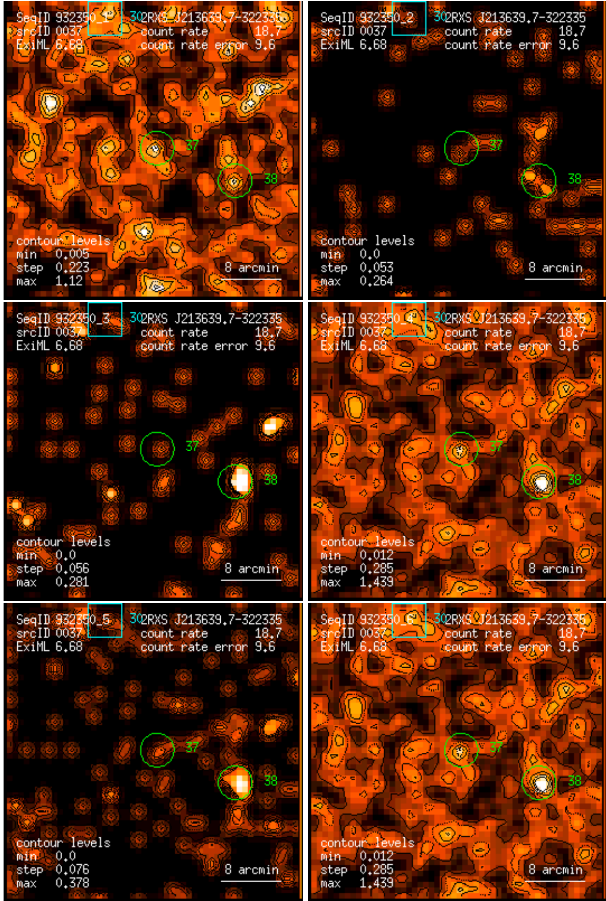
Figure 37: RASS 932350: detection 0037: band rate images, Gaussian filter: (1) PSPC channels 11 – 41, (2) 52 – 90, (3) 91 – 201, (4) 11 – 235, (5) 52 – 201, (6) 11 – 201. Broad band rates in counts/ks. Band rate contour levels in counts/ks/arcmin 2 .
