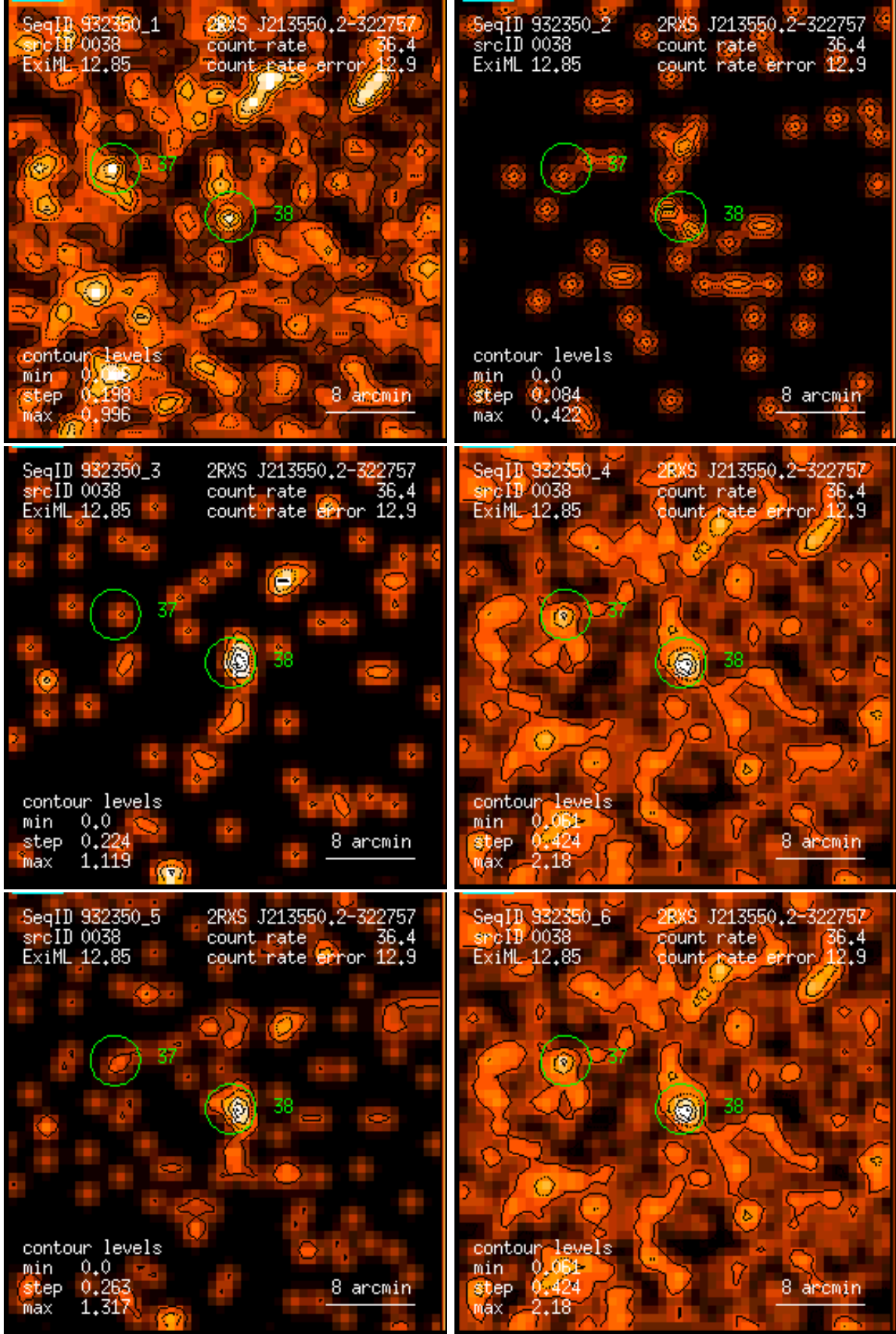
Figure 38: RASS 932350: detection 0038: band rate images, Gaussian filter: (1) PSPC channels 11 – 41, (2) 52 – 90, (3) 91 – 201, (4) 11 – 235, (5) 52 – 201, (6) 11 – 201. Broad band rates in counts/ks. Band rate contour levels in counts/ks/arcmin 2 .
