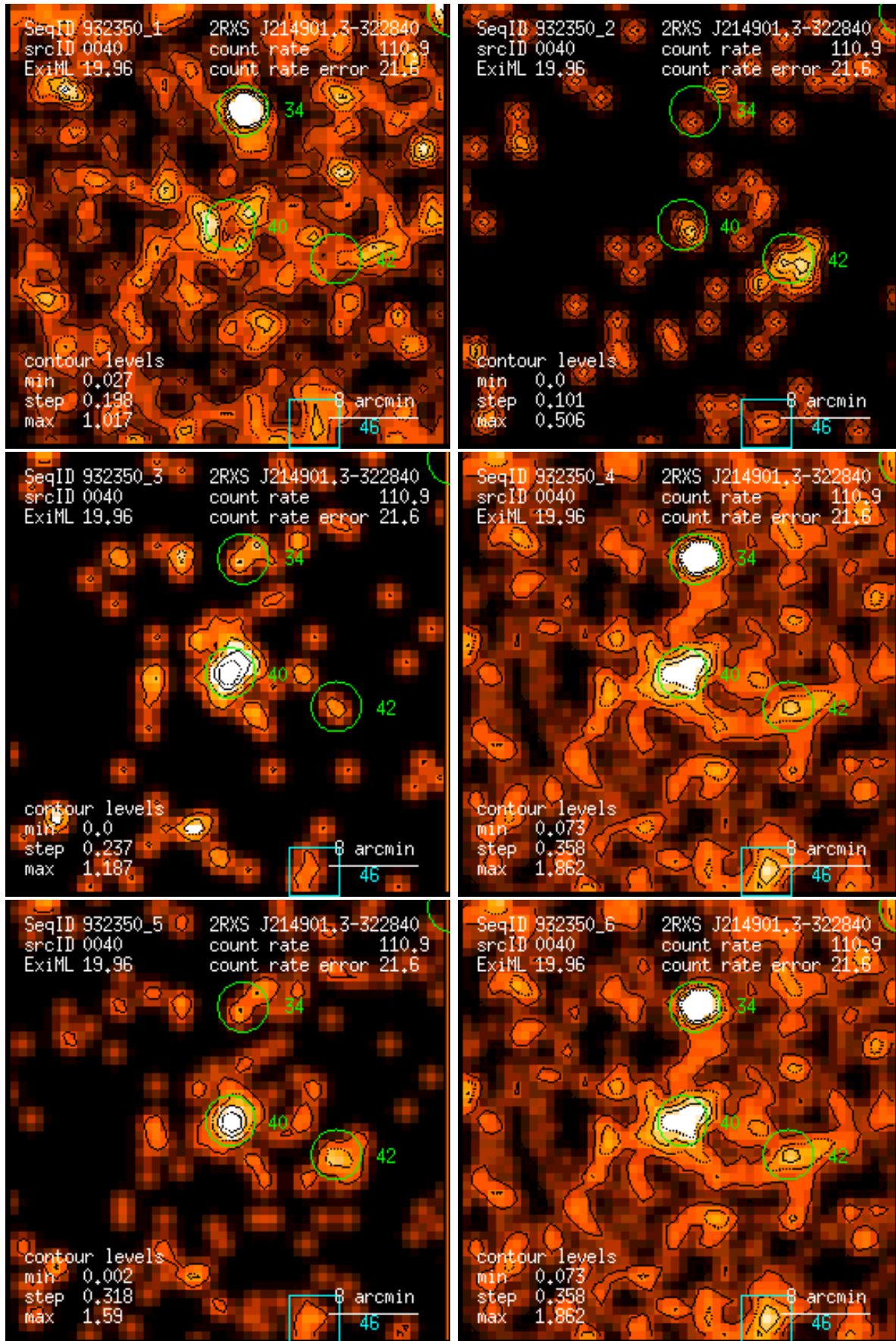
Figure 40: RASS 932350: detection 0040: band rate images, Gaussian filter: (1) PSPC channels 11 – 41, (2) 52 – 90, (3) 91 – 201, (4) 11 – 235, (5) 52 – 201, (6) 11 – 201. Broad band rates in counts/ks. Band rate contour levels in counts/ks/arcmin 2 .
