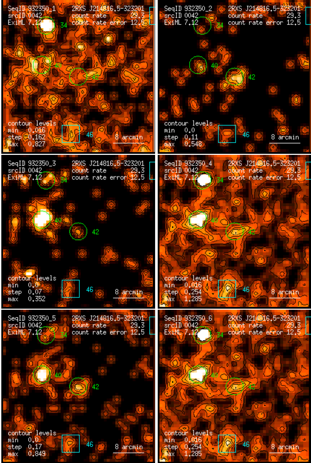
Figure 42: RASS 932350: detection 0042: band rate images, Gaussian filter: (1) PSPC channels 11 – 41, (2) 52 – 90, (3) 91 – 201, (4) 11 – 235, (5) 52 – 201, (6) 11 – 201. Broad band rates in counts/ks. Band rate contour levels in counts/ks/arcmin 2 .
