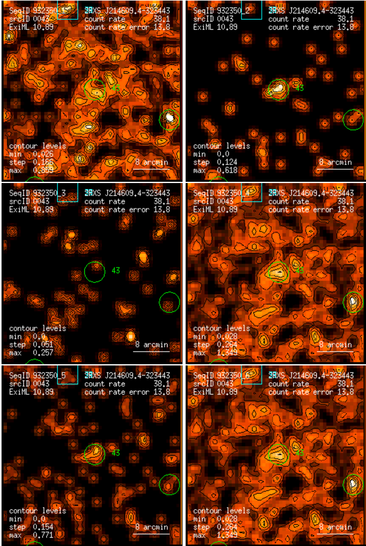
Figure 43: RASS 932350: detection 0043: band rate images, Gaussian filter: (1) PSPC channels 11 – 41, (2) 52 – 90, (3) 91 – 201, (4) 11 – 235, (5) 52 – 201, (6) 11 – 201. Broad band rates in counts/ks. Band rate contour levels in counts/ks/arcmin 2 .
