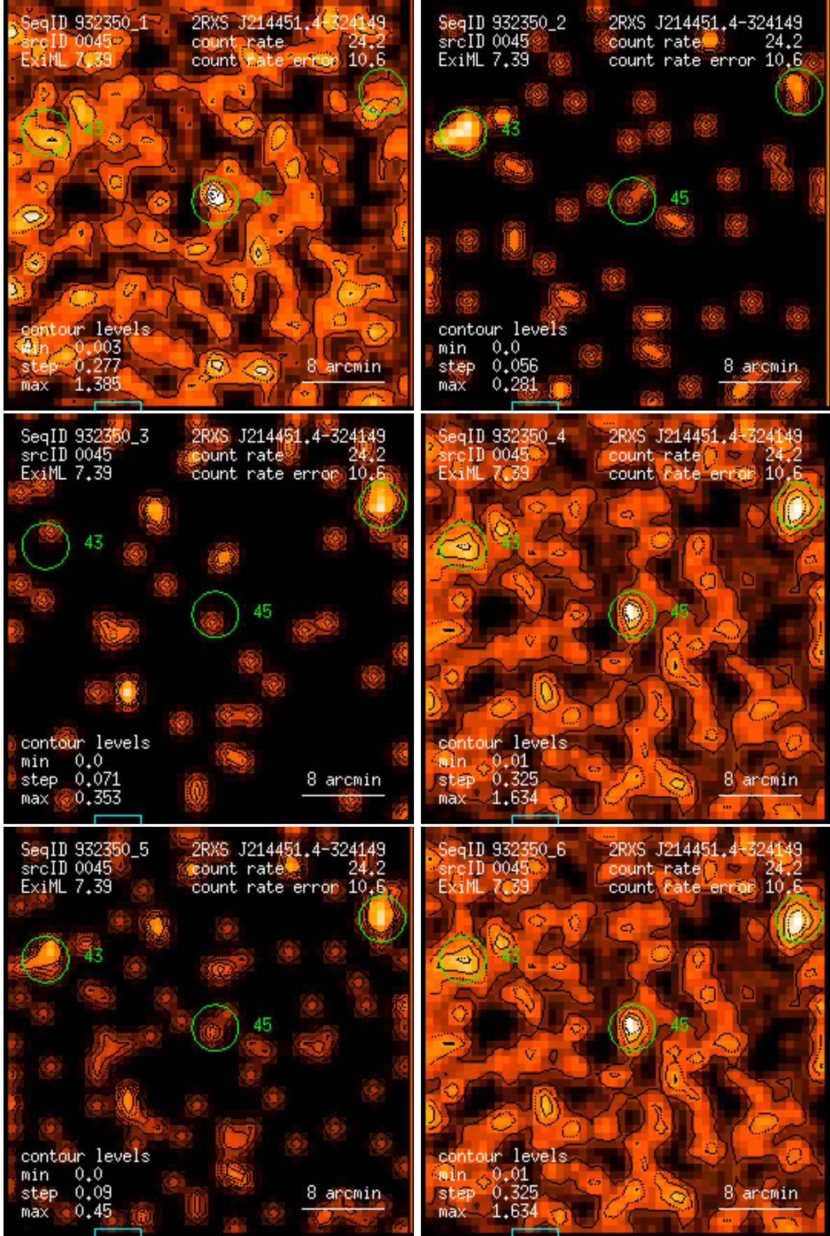
Figure 45: RASS 932350: detection 0045: band rate images, Gaussian filter: (1) PSPC channels 11 – 41, (2) 52 – 90, (3) 91 – 201, (4) 11 – 235, (5) 52 – 201, (6) 11 – 201. Broad band rates in counts/ks. Band rate contour levels in counts/ks/arcmin 2 .
