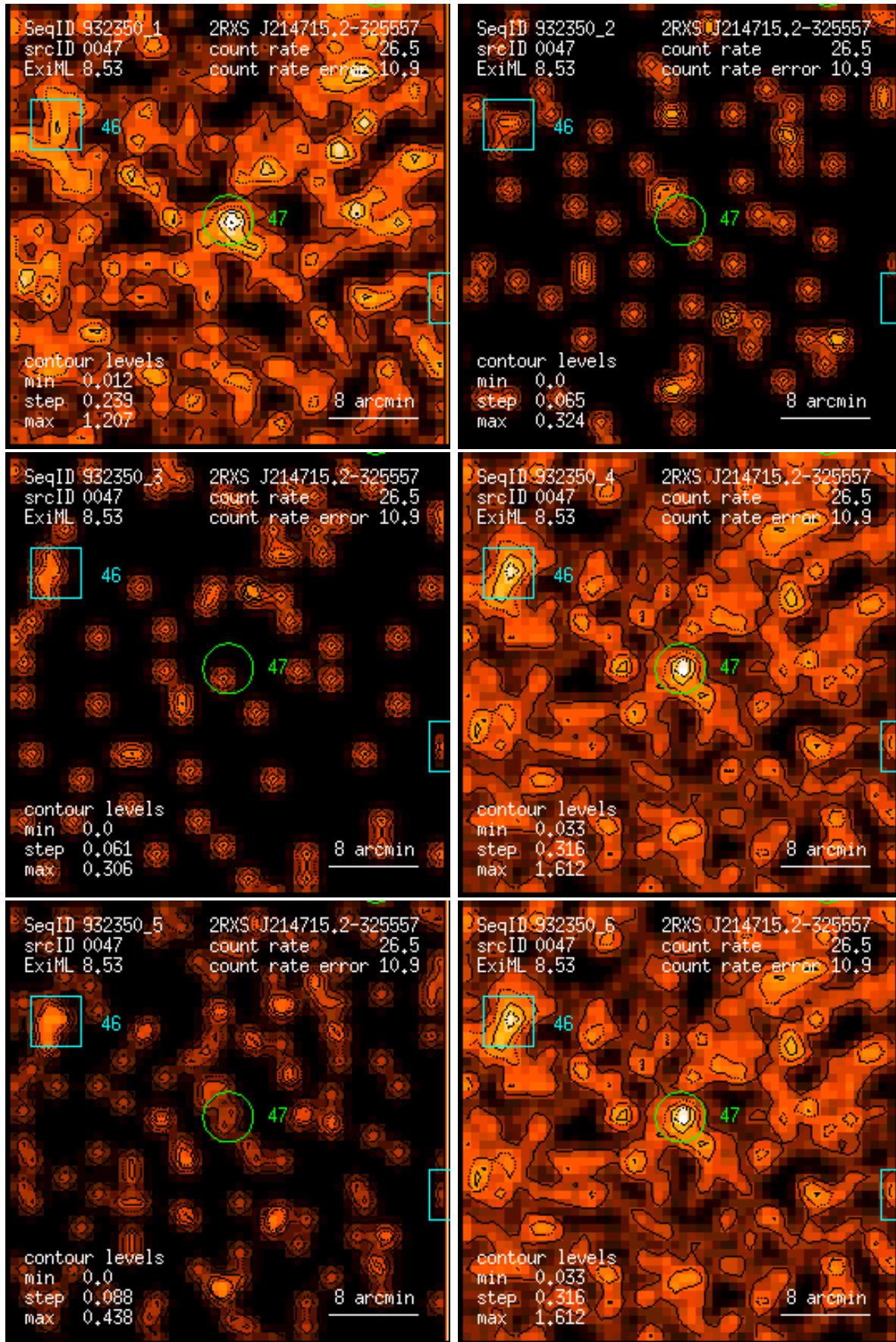
Figure 47: RASS 932350: detection 0047: band rate images, Gaussian filter: (1) PSPC channels 11 – 41, (2) 52 – 90, (3) 91 – 201, (4) 11 – 235, (5) 52 – 201, (6) 11 – 201. Broad band rates in counts/ks. Band rate contour levels in counts/ks/arcmin 2 .
