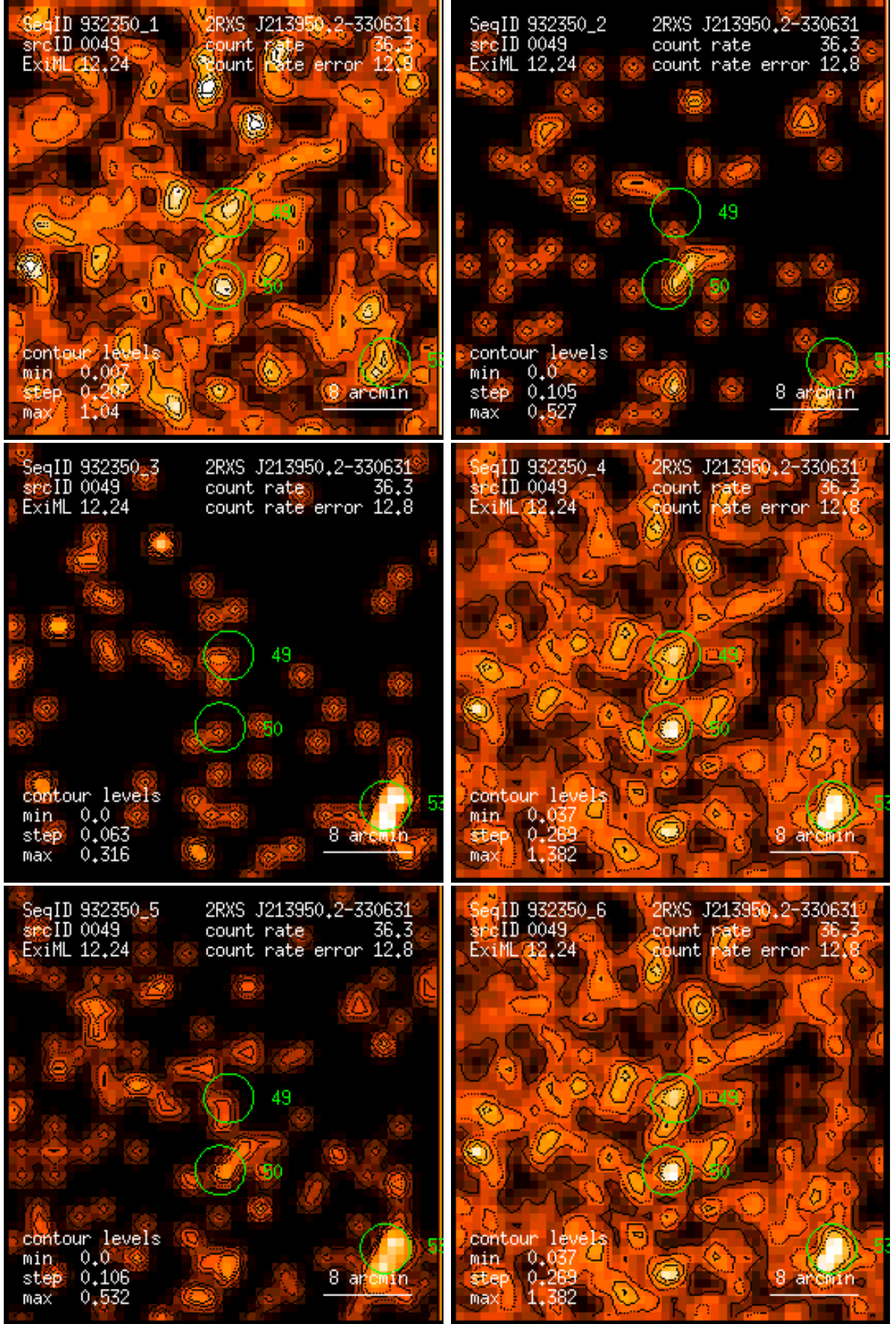
Figure 49: RASS 932350: detection 0049: band rate images, Gaussian filter: (1) PSPC channels 11 – 41, (2) 52 – 90, (3) 91 – 201, (4) 11 – 235, (5) 52 – 201, (6) 11 – 201. Broad band rates in counts/ks. Band rate contour levels in counts/ks/arcmin 2 .
