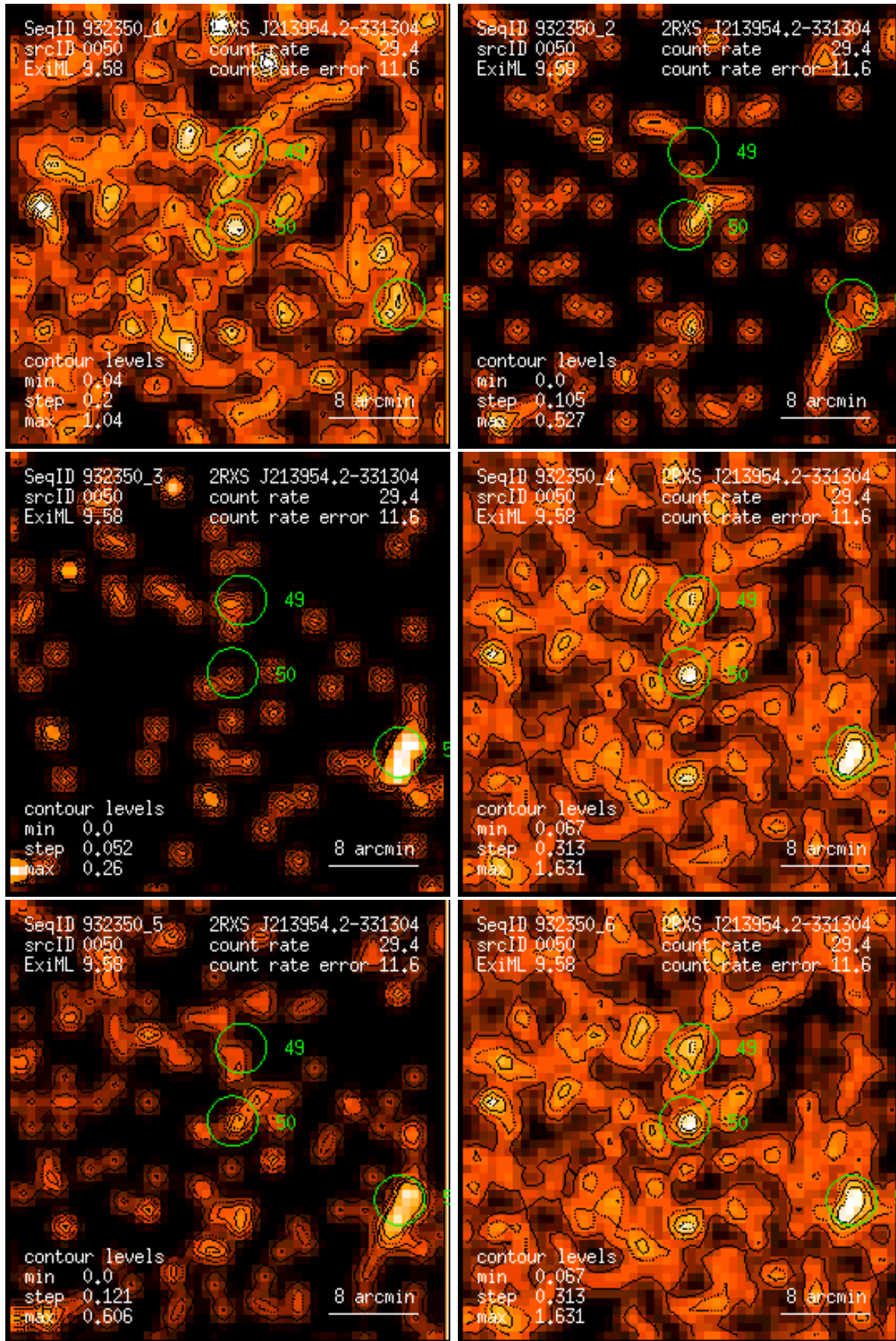
Figure 50: RASS 932350: detection 0050: band rate images, Gaussian filter: (1) PSPC channels 11 – 41, (2) 52 – 90, (3) 91 – 201, (4) 11 – 235, (5) 52 – 201, (6) 11 – 201. Broad band rates in counts/ks. Band rate contour levels in counts/ks/arcmin 2 .
