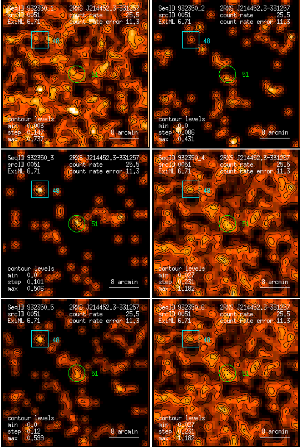
Figure 51: RASS 932350: detection 0051: band rate images, Gaussian filter: (1) PSPC channels 11 – 41, (2) 52 – 90, (3) 91 – 201, (4) 11 – 235, (5) 52 – 201, (6) 11 – 201. Broad band rates in counts/ks. Band rate contour levels in counts/ks/arcmin 2 .
