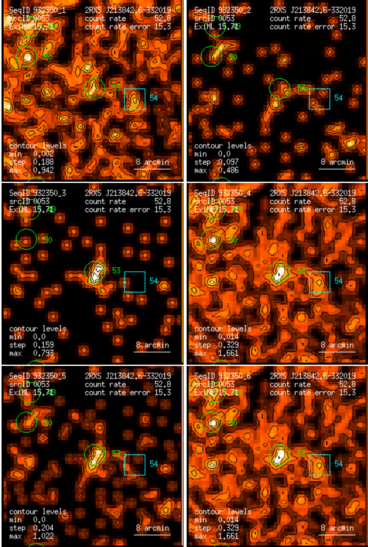
Figure 53: RASS 932350: detection 0053: band rate images, Gaussian filter: (1) PSPC channels 11 – 41, (2) 52 – 90, (3) 91 – 201, (4) 11 – 235, (5) 52 – 201, (6) 11 – 201. Broad band rates in counts/ks. Band rate contour levels in counts/ks/arcmin 2 .
