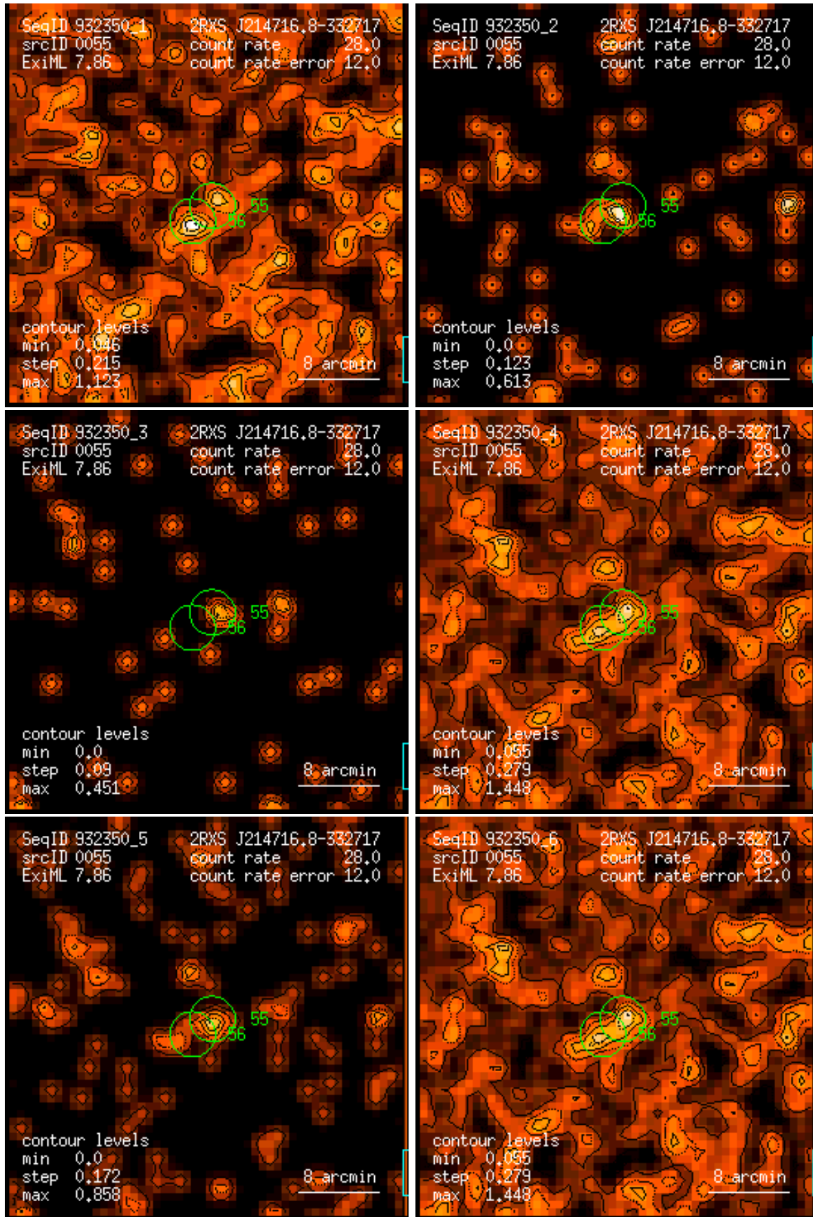
Figure 55: RASS 932350: detection 0055: band rate images, Gaussian filter: (1) PSPC channels 11 – 41, (2) 52 – 90, (3) 91 – 201, (4) 11 – 235, (5) 52 – 201, (6) 11 – 201. Broad band rates in counts/ks. Band rate contour levels in counts/ks/arcmin 2 .
