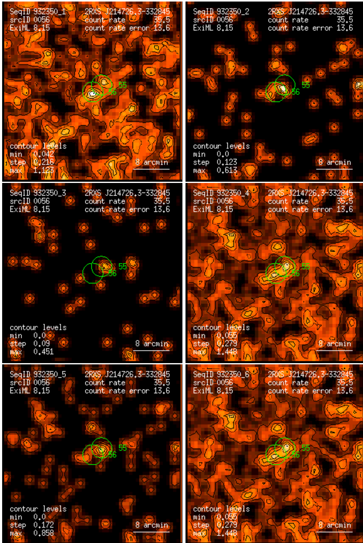
Figure 56: RASS 932350: detection 0056: band rate images, Gaussian filter: (1) PSPC channels 11 – 41, (2) 52 – 90, (3) 91 – 201, (4) 11 – 235, (5) 52 – 201, (6) 11 – 201. Broad band rates in counts/ks. Band rate contour levels in counts/ks/arcmin 2 .
