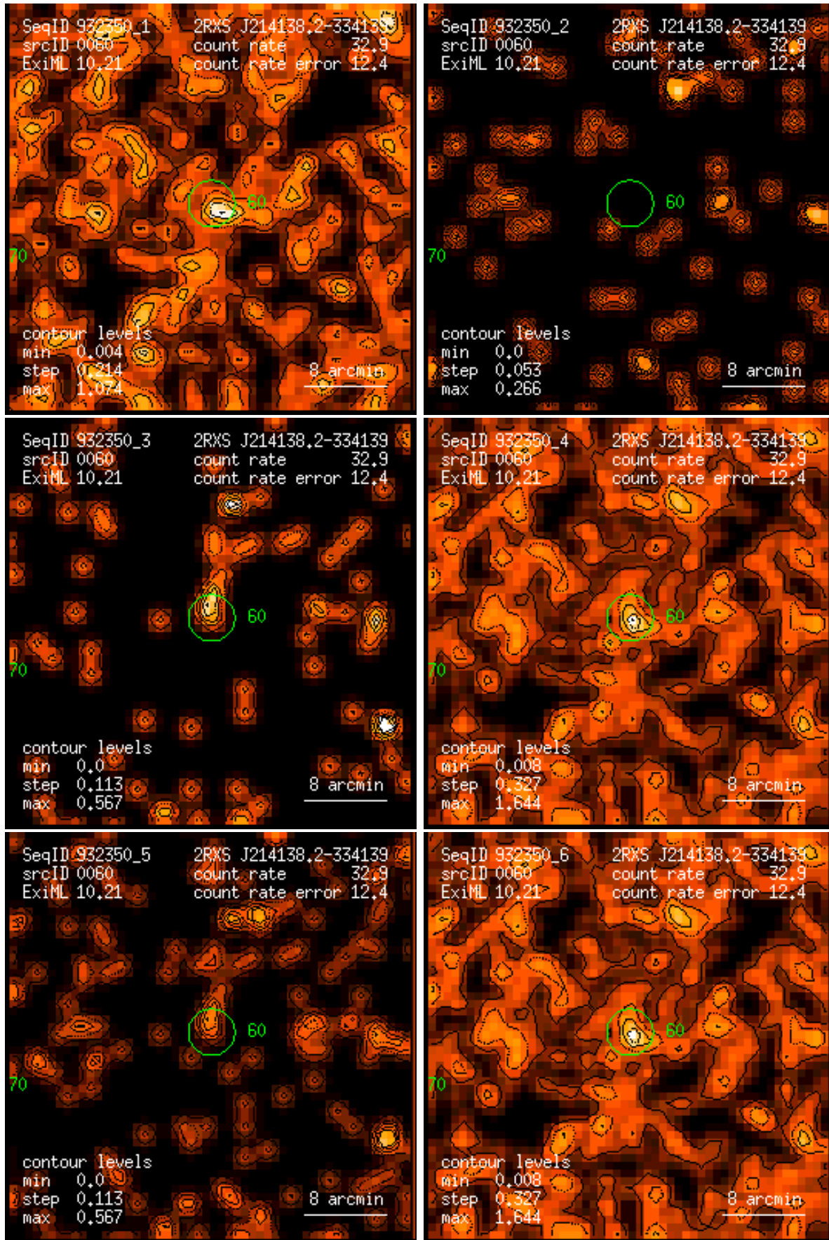
Figure 60: RASS 932350: detection 0060: band rate images, Gaussian filter: (1) PSPC channels 11 – 41, (2) 52 – 90, (3) 91 – 201, (4) 11 – 235, (5) 52 – 201, (6) 11 – 201. Broad band rates in counts/ks. Band rate contour levels in counts/ks/arcmin 2 .
