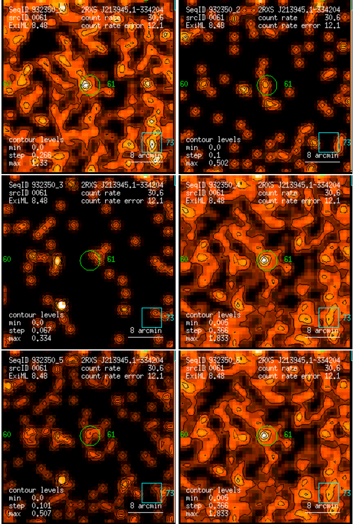
Figure 61: RASS 932350: detection 0061: band rate images, Gaussian filter: (1) PSPC channels 11 – 41, (2) 52 – 90, (3) 91 – 201, (4) 11 – 235, (5) 52 – 201, (6) 11 – 201. Broad band rates in counts/ks. Band rate contour levels in counts/ks/arcmin 2 .
