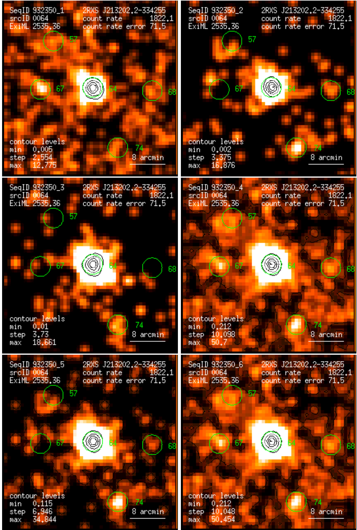
Figure 64: RASS 932350: detection 0064: band rate images, Gaussian filter: (1) PSPC channels 11 – 41, (2) 52 – 90, (3) 91 – 201, (4) 11 – 235, (5) 52 – 201, (6) 11 – 201. Broad band rates in counts/ks. Band rate contour levels in counts/ks/arcmin 2 .
