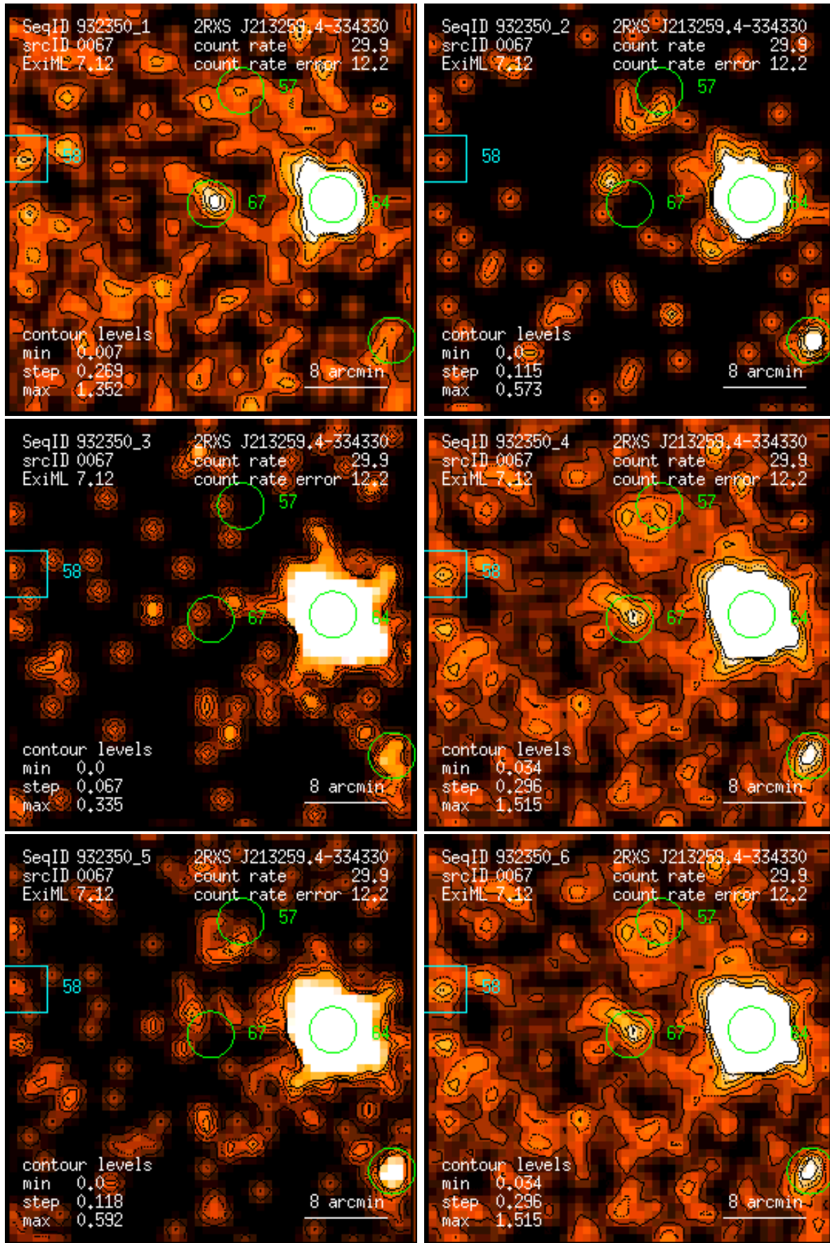
Figure 67: RASS 932350: detection 0067: band rate images, Gaussian filter: (1) PSPC channels 11 – 41, (2) 52 – 90, (3) 91 – 201, (4) 11 – 235, (5) 52 – 201, (6) 11 – 201. Broad band rates in counts/ks. Band rate contour levels in counts/ks/arcmin 2 .
