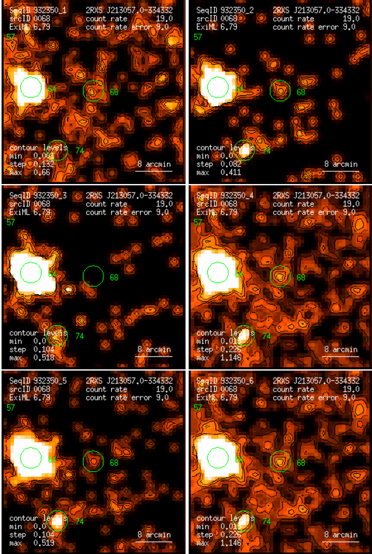
Figure 68: RASS 932350: detection 0068: band rate images, Gaussian filter: (1) PSPC channels 11 – 41, (2) 52 – 90, (3) 91 – 201, (4) 11 – 235, (5) 52 – 201, (6) 11 – 201. Broad band rates in counts/ks. Band rate contour levels in counts/ks/arcmin 2 .
