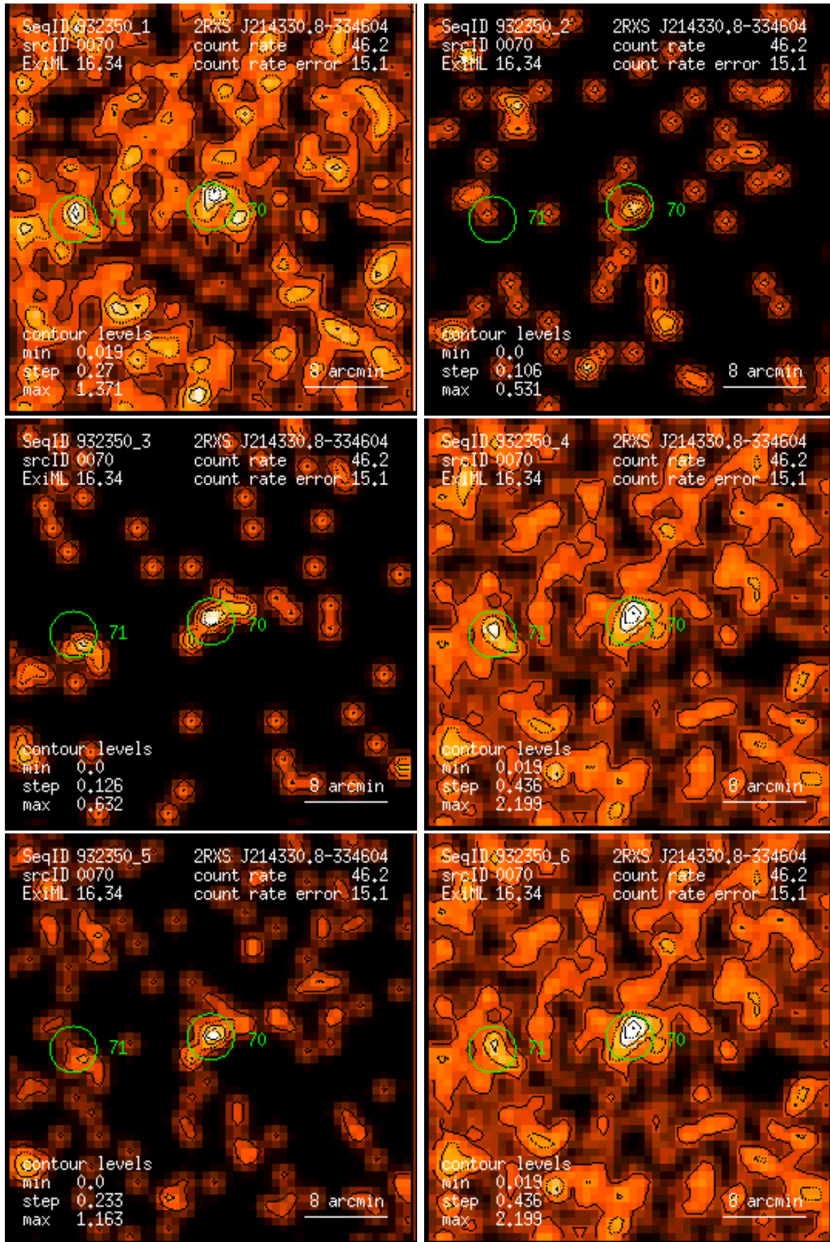
Figure 70: RASS 932350: detection 0070: band rate images, Gaussian filter: (1) PSPC channels 11 – 41, (2) 52 – 90, (3) 91 – 201, (4) 11 – 235, (5) 52 – 201, (6) 11 – 201. Broad band rates in counts/ks. Band rate contour levels in counts/ks/arcmin 2 .
