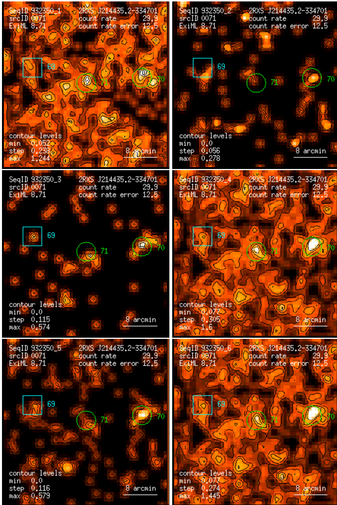
Figure 71: RASS 932350: detection 0071: band rate images, Gaussian filter: (1) PSPC channels 11 – 41, (2) 52 – 90, (3) 91 – 201, (4) 11 – 235, (5) 52 – 201, (6) 11 – 201. Broad band rates in counts/ks. Band rate contour levels in counts/ks/arcmin 2 .
