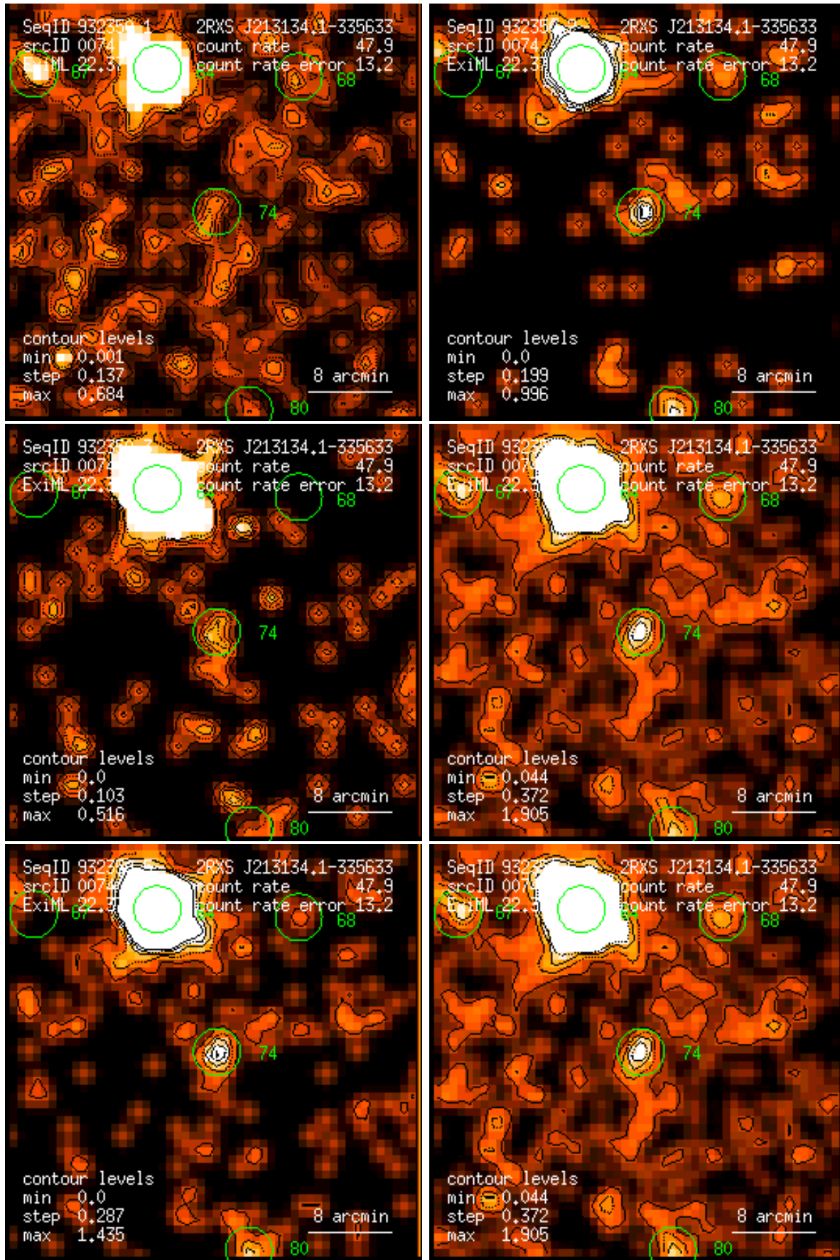
Figure 74: RASS 932350: detection 0074: band rate images, Gaussian filter: (1) PSPC channels 11 – 41, (2) 52 – 90, (3) 91 – 201, (4) 11 – 235, (5) 52 – 201, (6) 11 – 201. Broad band rates in counts/ks. Band rate contour levels in counts/ks/arcmin 2 .
