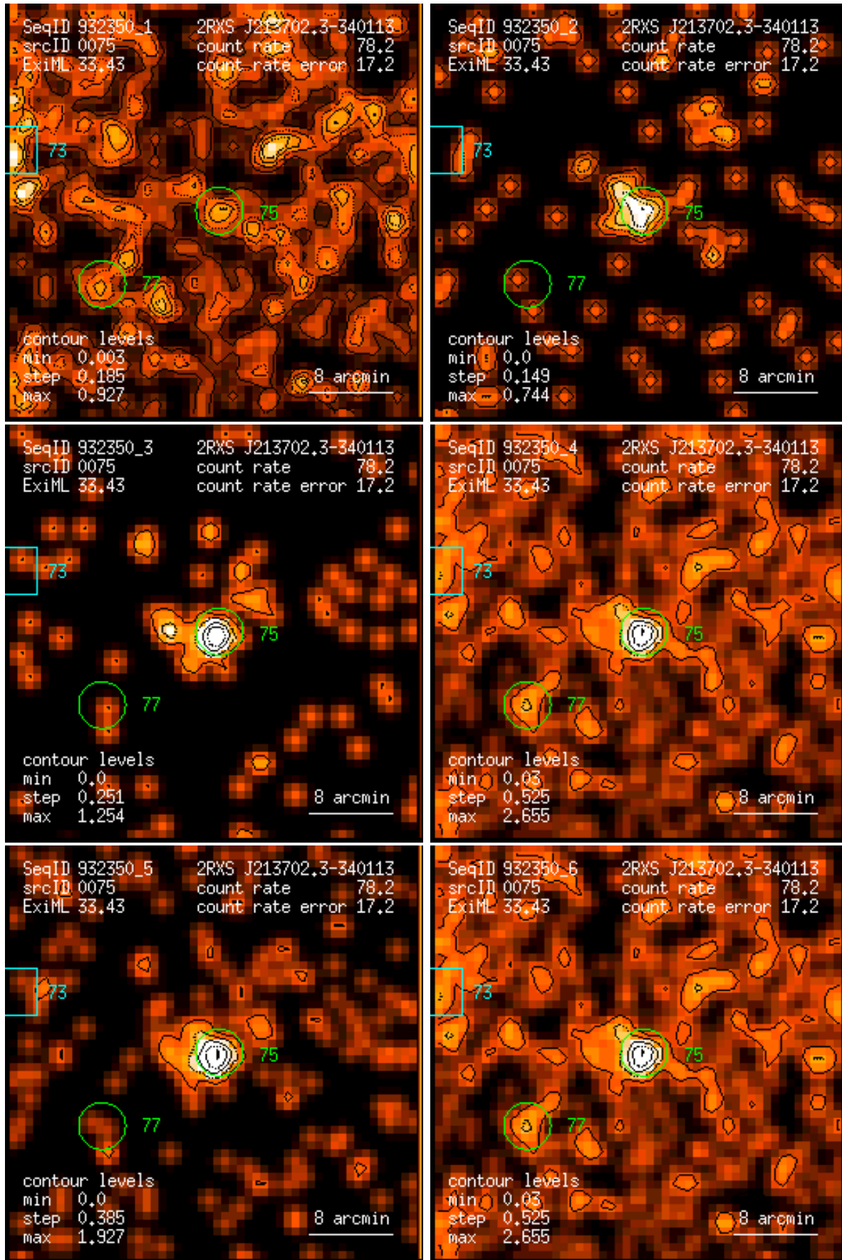
Figure 75: RASS 932350: detection 0075: band rate images, Gaussian filter: (1) PSPC channels 11 – 41, (2) 52 – 90, (3) 91 – 201, (4) 11 – 235, (5) 52 – 201, (6) 11 – 201. Broad band rates in counts/ks. Band rate contour levels in counts/ks/arcmin 2 .
