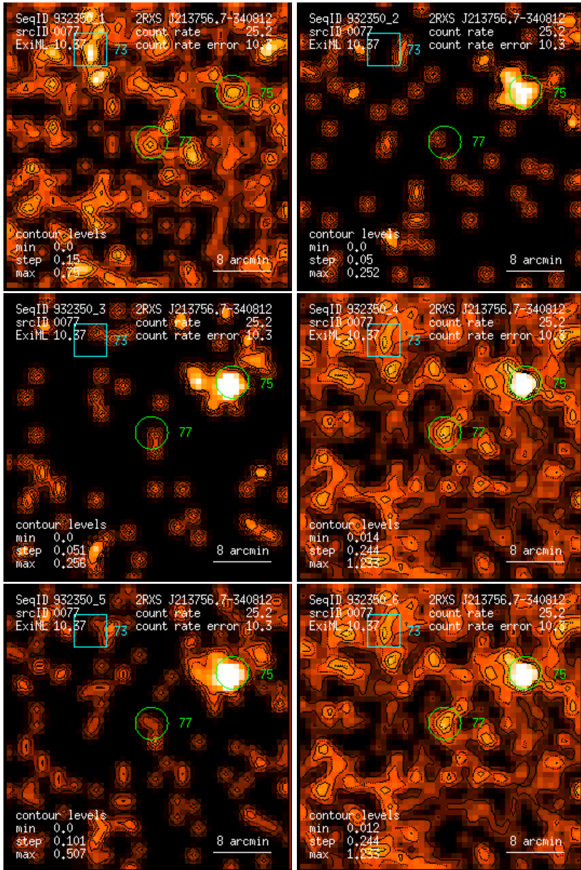
Figure 77: RASS 932350: detection 0077: band rate images, Gaussian filter: (1) PSPC channels 11 – 41, (2) 52 – 90, (3) 91 – 201, (4) 11 – 235, (5) 52 – 201, (6) 11 – 201. Broad band rates in counts/ks. Band rate contour levels in counts/ks/arcmin 2 .
