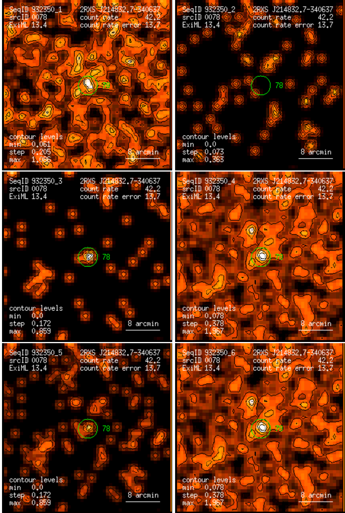
Figure 78: RASS 932350: detection 0078: band rate images, Gaussian filter: (1) PSPC channels 11 – 41, (2) 52 – 90, (3) 91 – 201, (4) 11 – 235, (5) 52 – 201, (6) 11 – 201. Broad band rates in counts/ks. Band rate contour levels in counts/ks/arcmin 2 .
