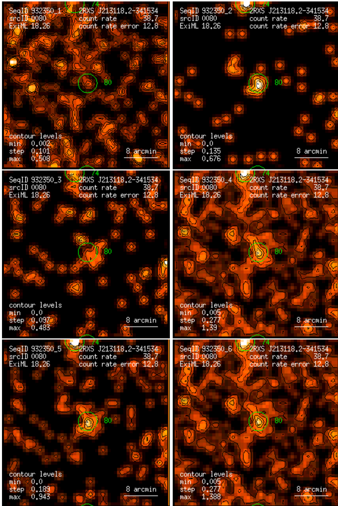
Figure 80: RASS 932350: detection 0080: band rate images, Gaussian filter: (1) PSPC channels 11 – 41, (2) 52 – 90, (3) 91 – 201, (4) 11 – 235, (5) 52 – 201, (6) 11 – 201. Broad band rates in counts/ks. Band rate contour levels in counts/ks/arcmin 2 .
