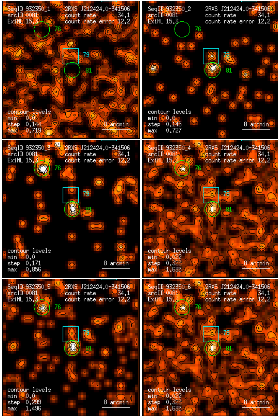
Figure 81: RASS 932350: detection 0081: band rate images, Gaussian filter: (1) PSPC channels 11 – 41, (2) 52 – 90, (3) 91 – 201, (4) 11 – 235, (5) 52 – 201, (6) 11 – 201. Broad band rates in counts/ks. Band rate contour levels in counts/ks/arcmin 2 .
