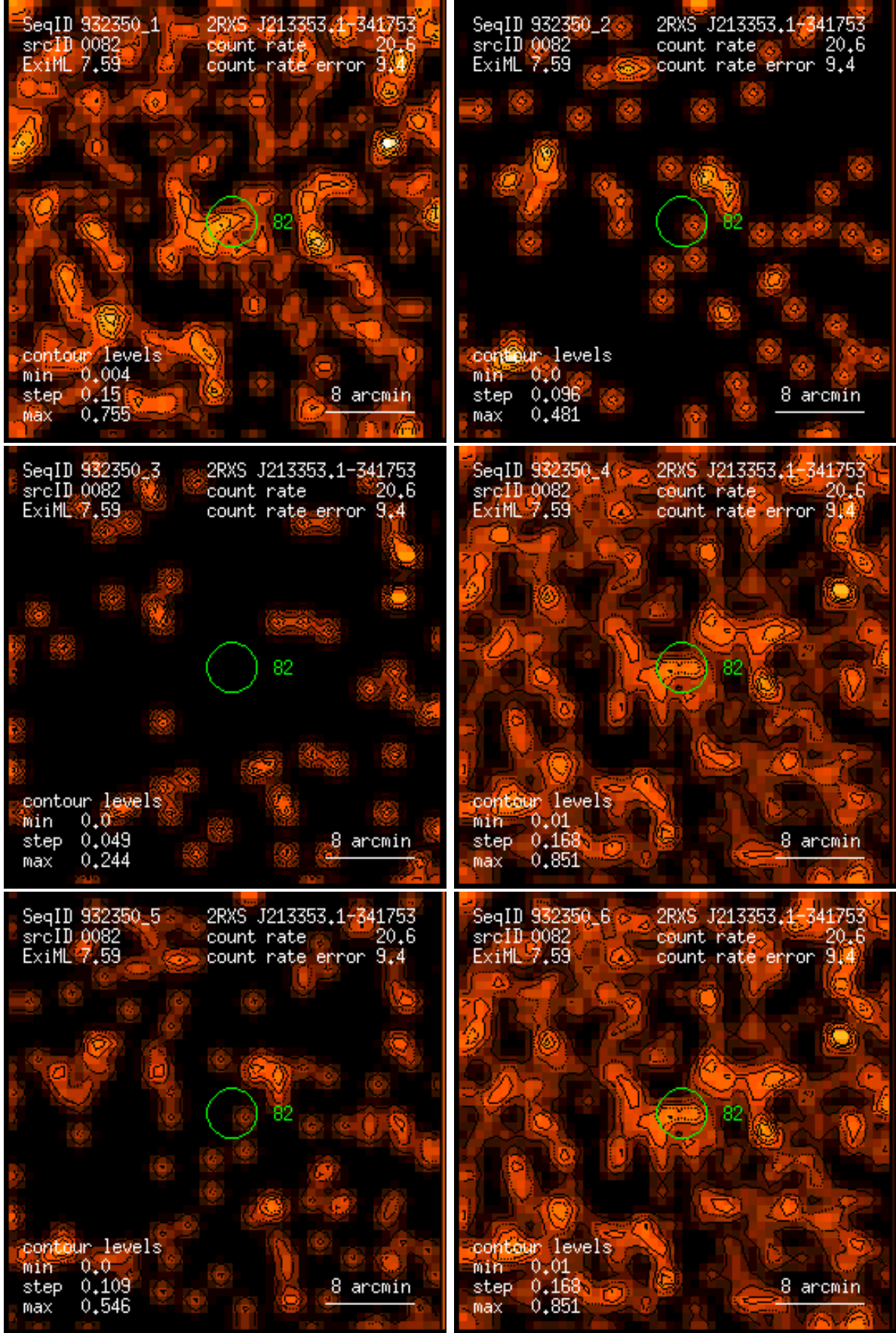
Figure 82: RASS 932350: detection 0082: band rate images, Gaussian filter: (1) PSPC channels 11 – 41, (2) 52 – 90, (3) 91 – 201, (4) 11 – 235, (5) 52 – 201, (6) 11 – 201. Broad band rates in counts/ks. Band rate contour levels in counts/ks/arcmin 2 .
