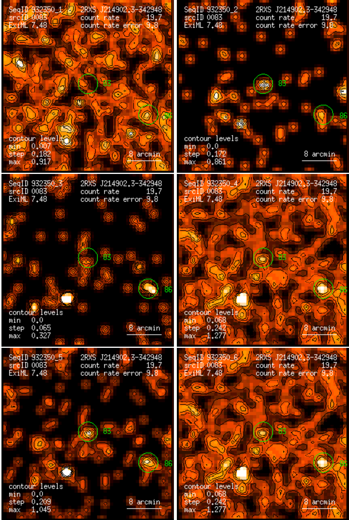
Figure 83: RASS 932350: detection 0083: band rate images, Gaussian filter: (1) PSPC channels 11 – 41, (2) 52 – 90, (3) 91 – 201, (4) 11 – 235, (5) 52 – 201, (6) 11 – 201. Broad band rates in counts/ks. Band rate contour levels in counts/ks/arcmin 2 .
