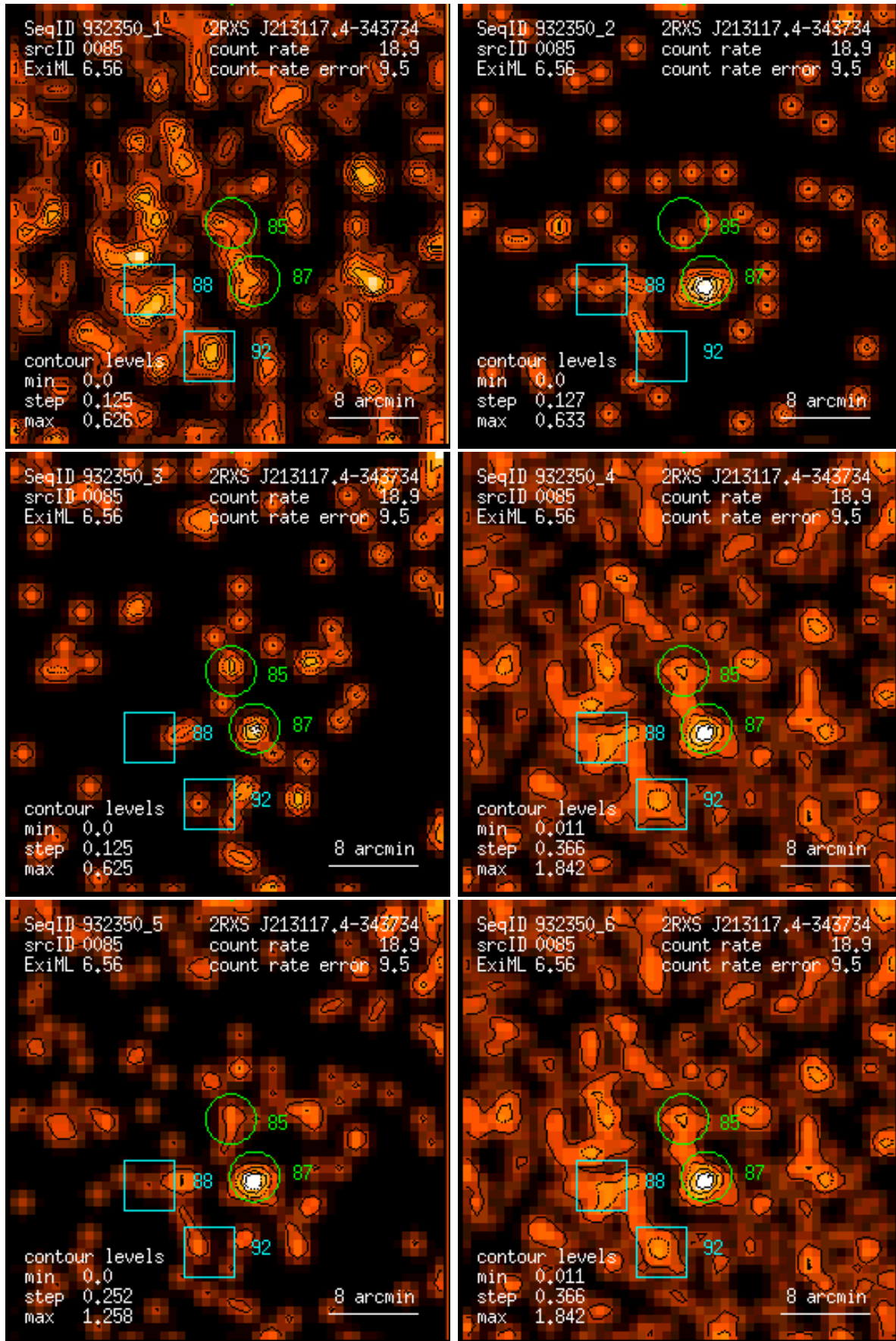
Figure 85: RASS 932350: detection 0085: band rate images, Gaussian filter: (1) PSPC channels 11 – 41, (2) 52 – 90, (3) 91 – 201, (4) 11 – 235, (5) 52 – 201, (6) 11 – 201. Broad band rates in counts/ks. Band rate contour levels in counts/ks/arcmin 2 .
