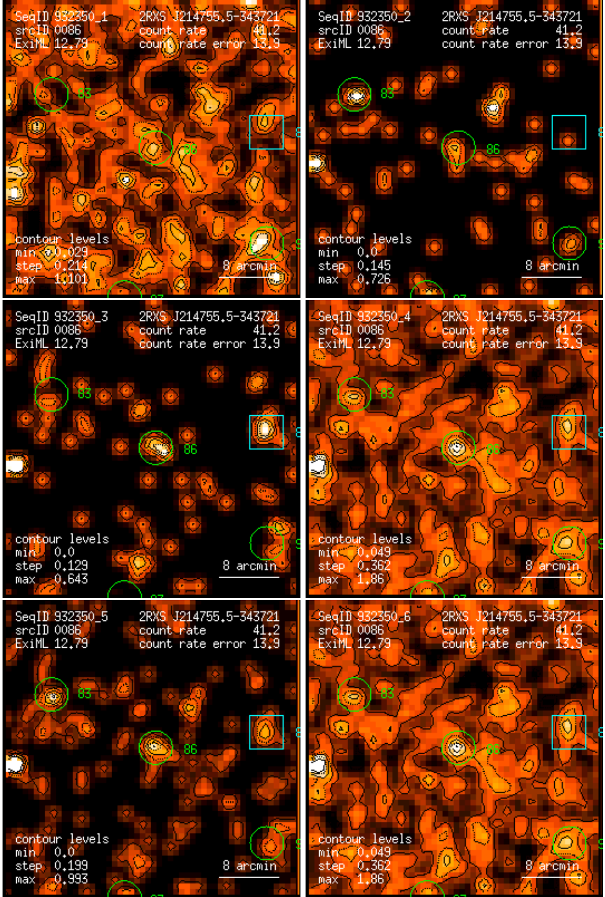
Figure 86: RASS 932350: detection 0086: band rate images, Gaussian filter: (1) PSPC channels 11 – 41, (2) 52 – 90, (3) 91 – 201, (4) 11 – 235, (5) 52 – 201, (6) 11 – 201. Broad band rates in counts/ks. Band rate contour levels in counts/ks/arcmin 2 .
